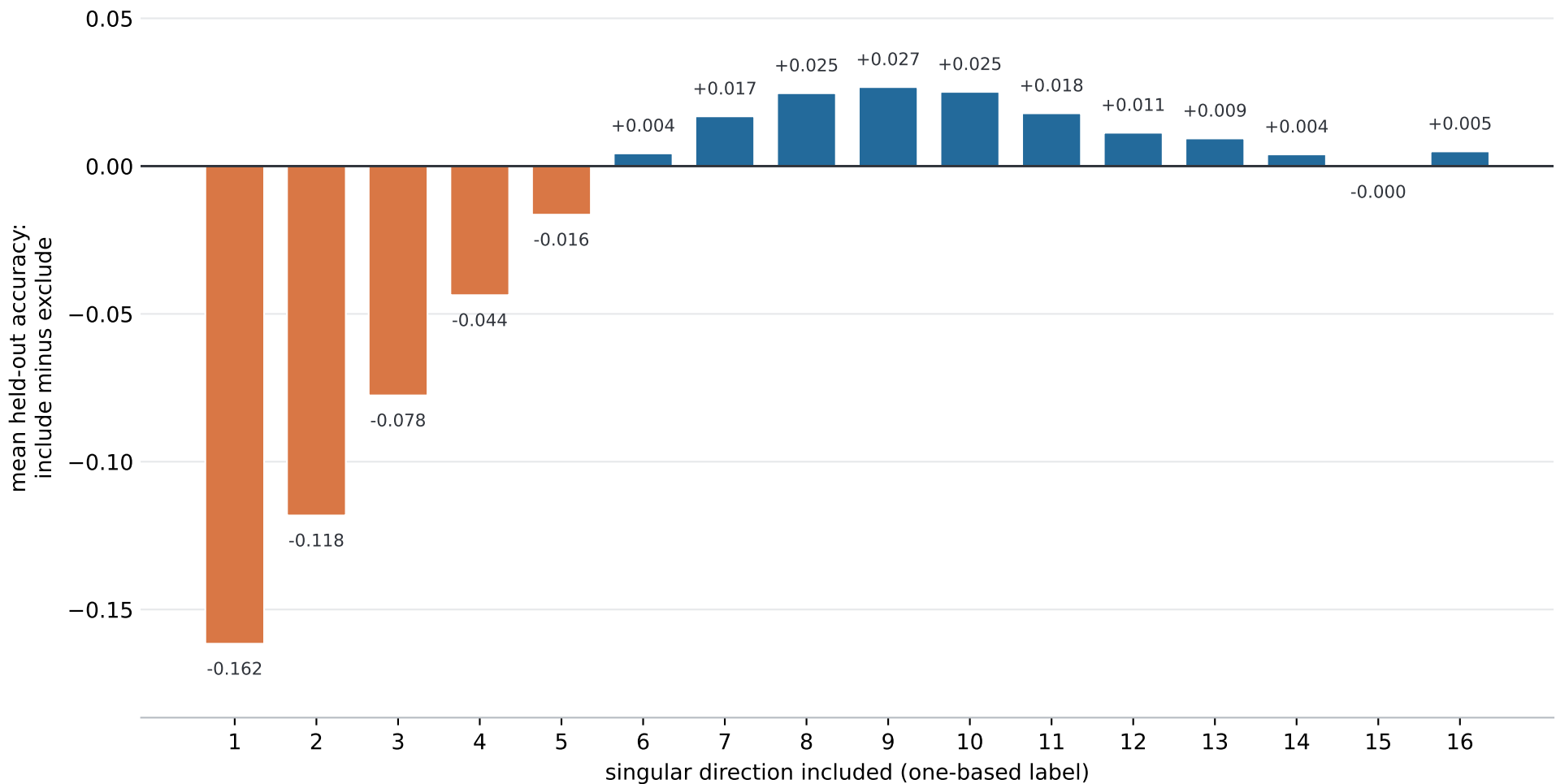
Qwen2.5-14B, MetaMathQA
