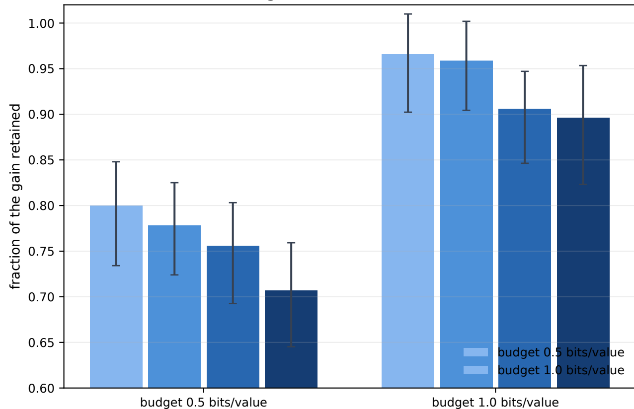
uniform beats every placement at a matched budget starving the late third hurts most
