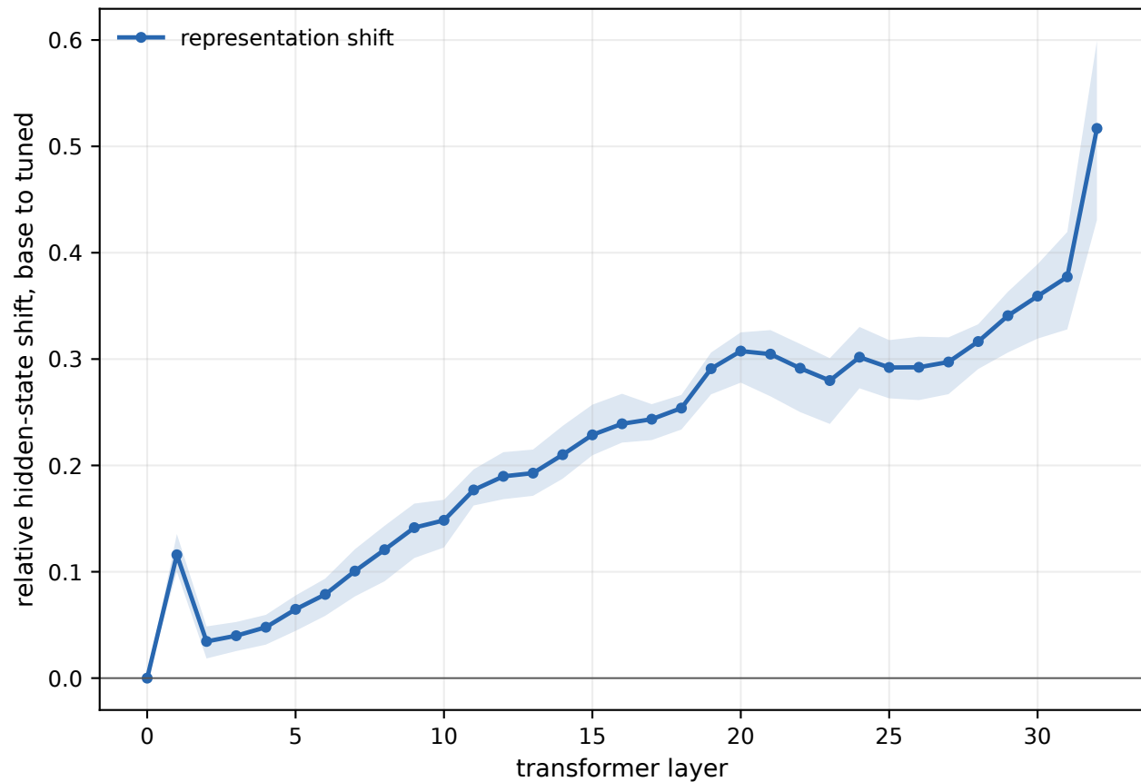
weights move evenly, the effect compounds with depth band is across arms and seeds
