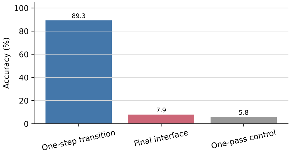
Small local errors compound over mixed h32 programs
