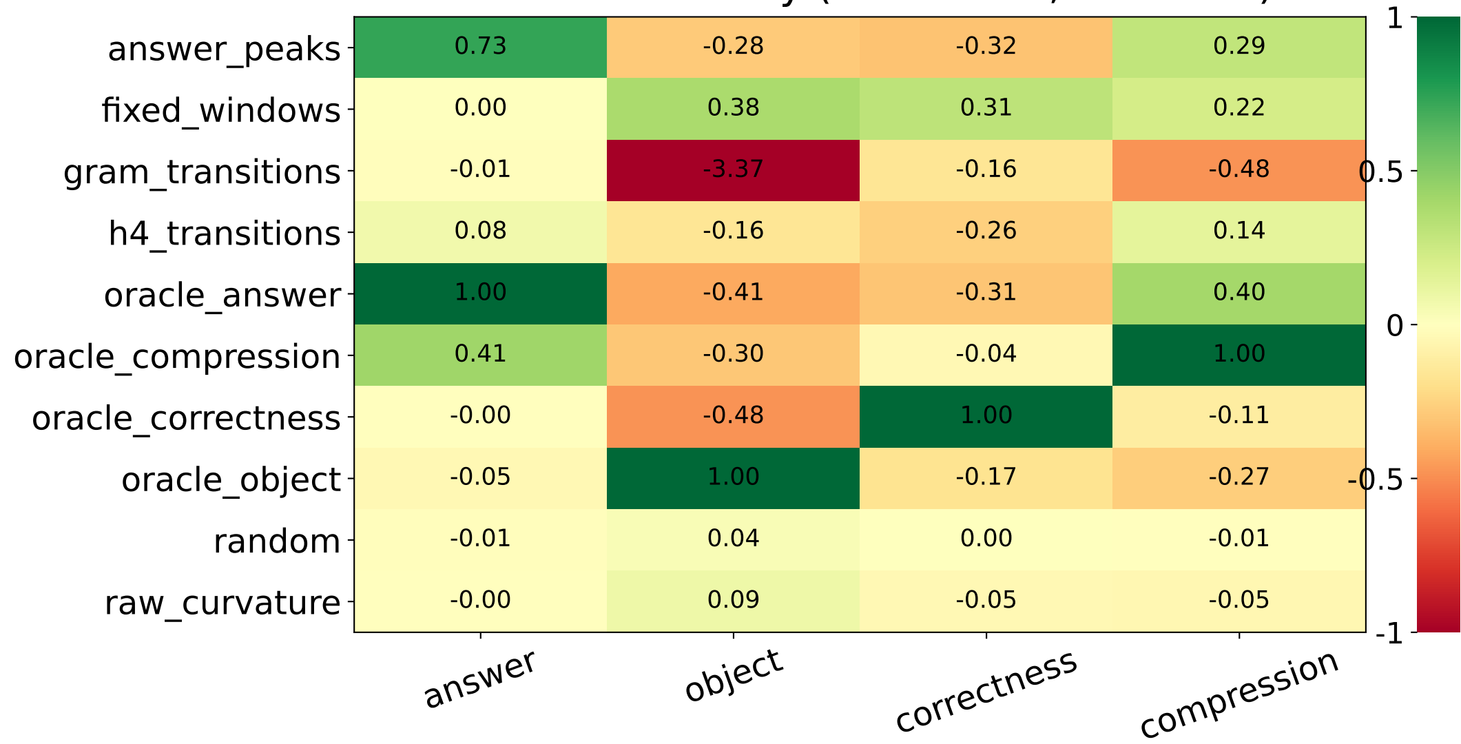
Normalized utility (random=0, oracle=1)
