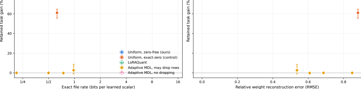
Figure 3: Adaptive MDL allocation against fixed-rate controls. Left: retained held-out prediction gain against exact decoded file rate. Right: retained gain against relative weight RMSE.
