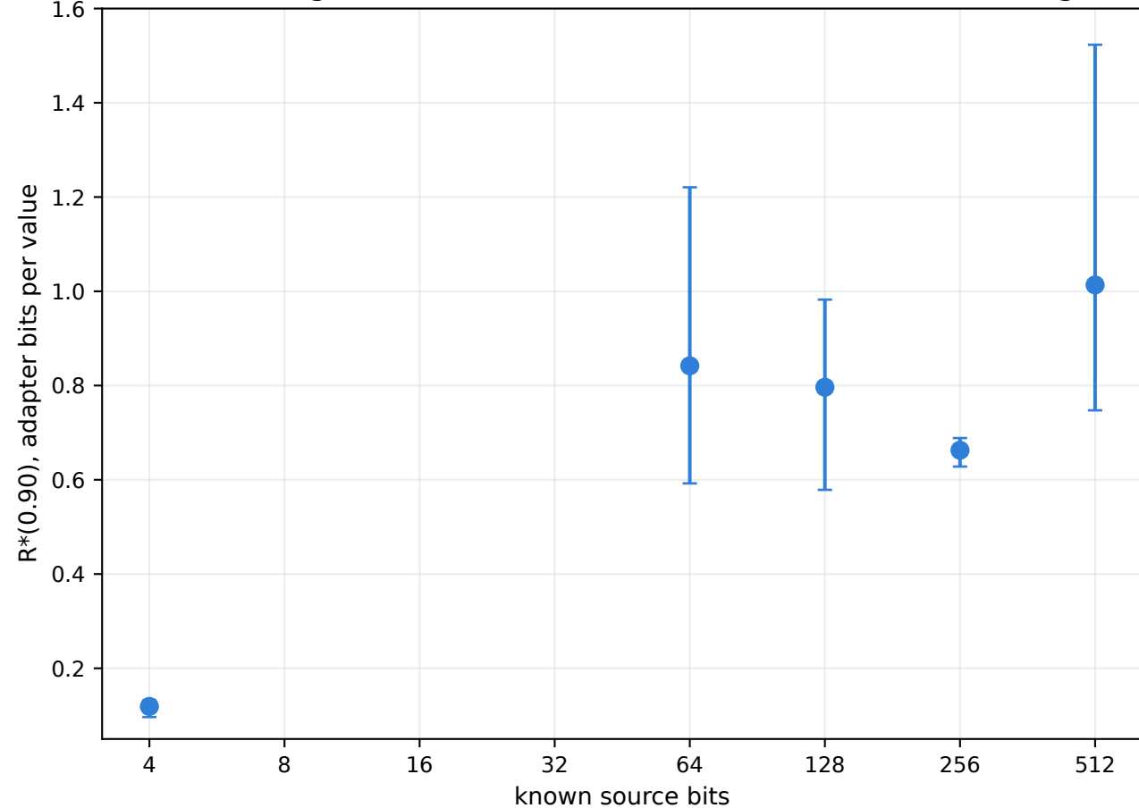
R^*(0.90) against known information, bars are the seed range
