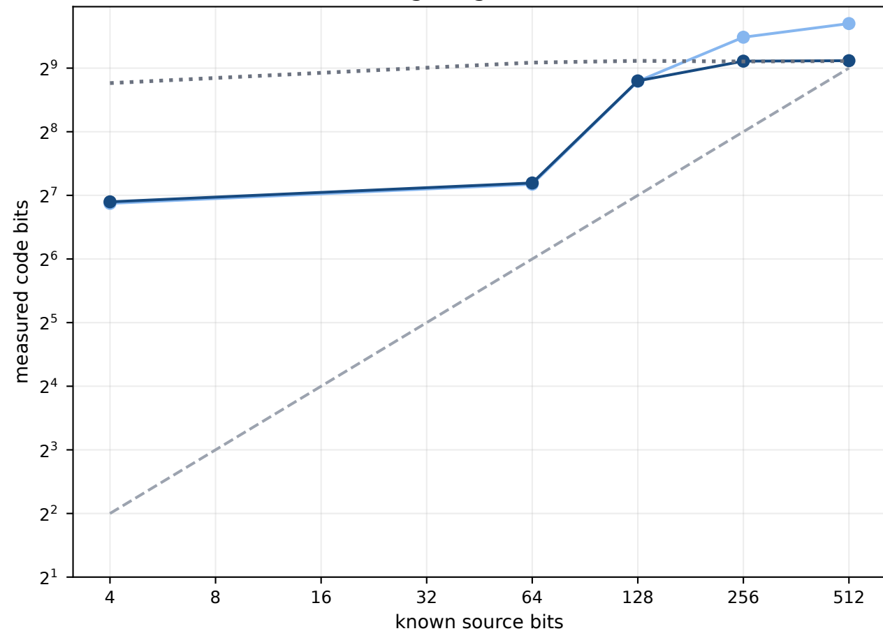
measured code length against known information
