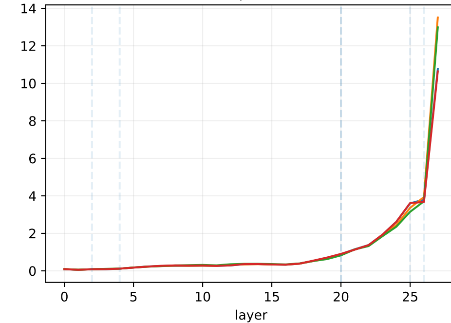
mlp rms
