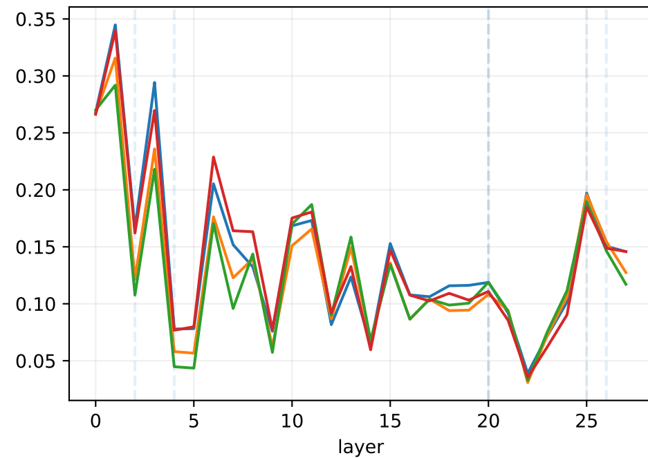
local attention 5
