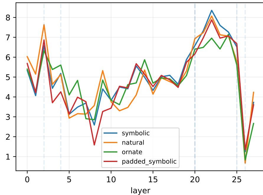
local attention 5
