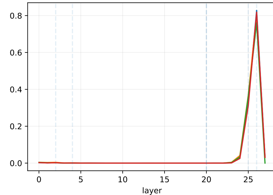
mlp rms
