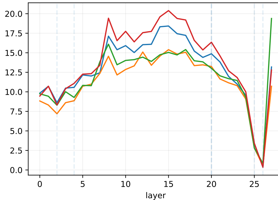
normalized update
