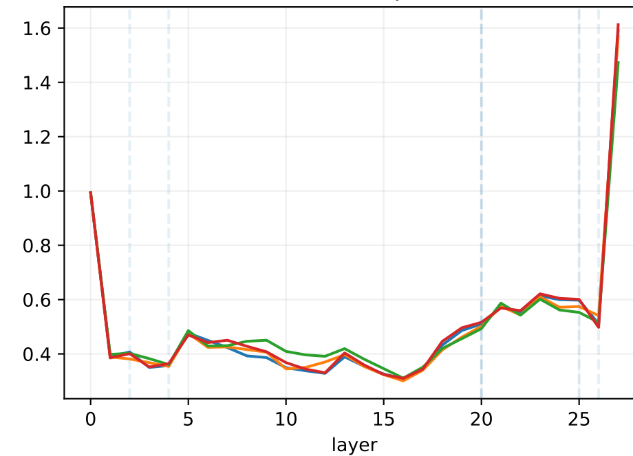
normalized update
