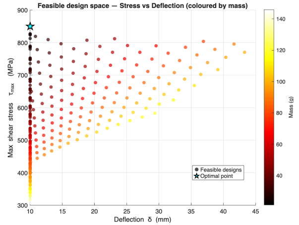
Figure 2: Feasible designs projected onto the stress-deflection plane and coloured by mass; the cyan star identifies the minimum-mass optimum, which trades maximum allowable stress for the smallest required deflection.
