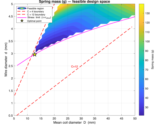
Figure 1: Spring mass (g) contour over the feasible ( D , d ) space; red dashed lines mark the manufacturability bounds C = 4 and C = 12 , the magenta curve is the stress limit, and the yellow star is the minimum-mass optimum.
