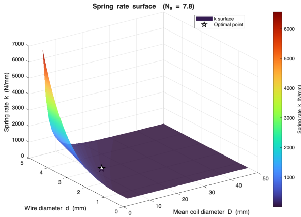
Figure 4: Spring rate k (N/mm) surface as a function of coil geometry at N_a = 7.77 ; the cubic inverse dependence on D causes a sharp stiffening as coil diameter decreases toward the C = 4 boundary.
