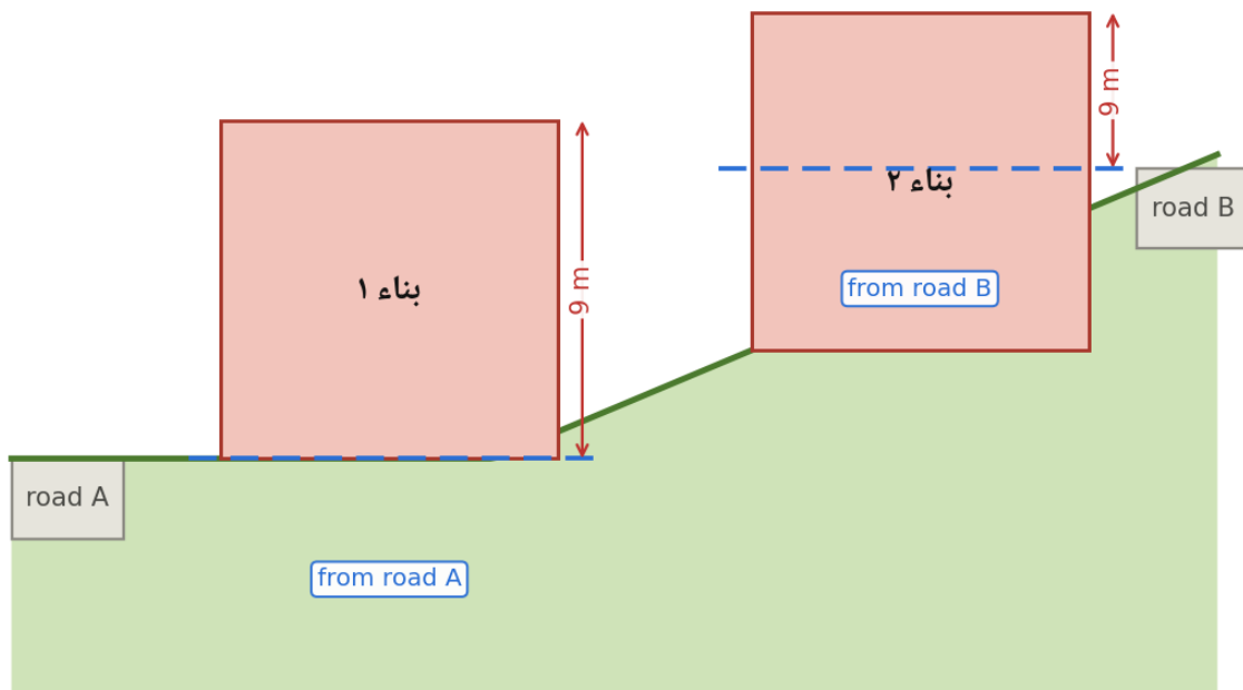
JO-Fig-06 — Several buildings — each takes the nearest road · Art 15(a)(3)
