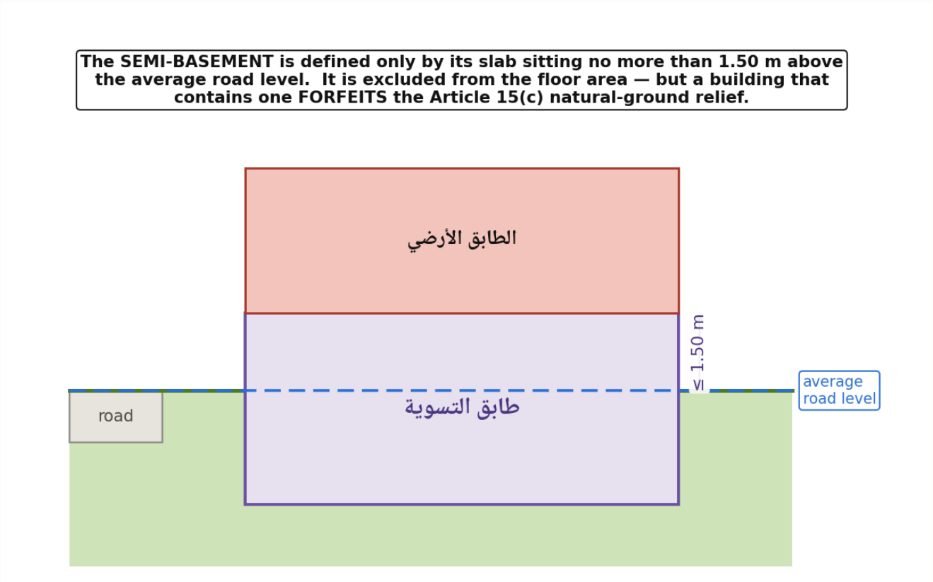
JO-Fig-11 — The semi-basement (تسوية) — the 1.50 m test, and what it costs · Art 2
