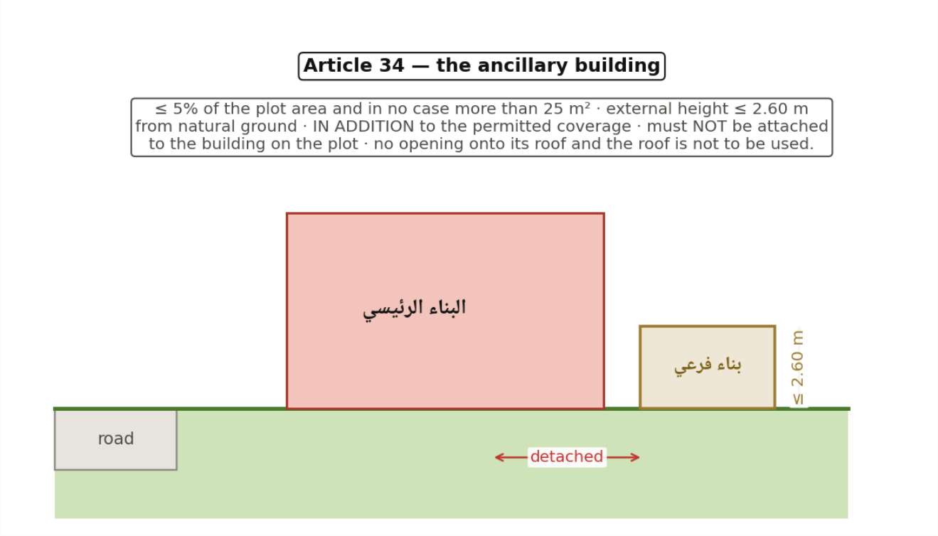
JO-Fig-24 — The ancillary building — additional to the coverage · Art 34
