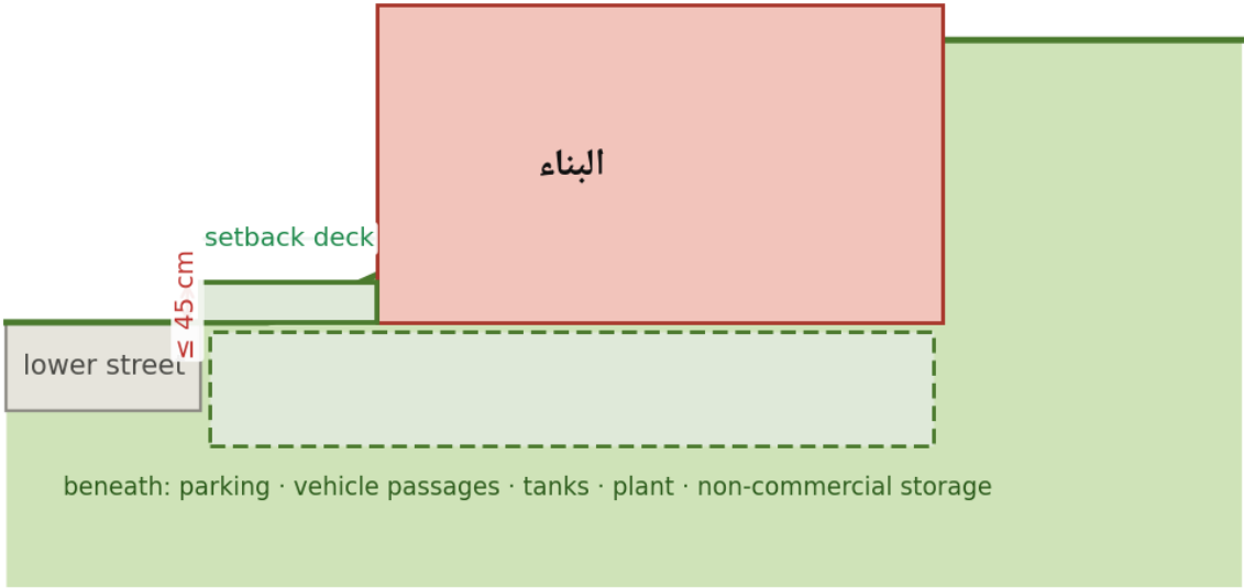
JO-Fig-23 — Decking the setbacks — excluded from both ratios · Art 33(d)
