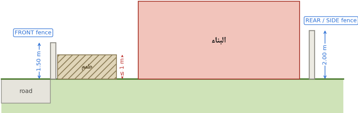
JO-Fig-22 — Fences and the 1 m cap on fill within the setbacks · Art 33(b)
