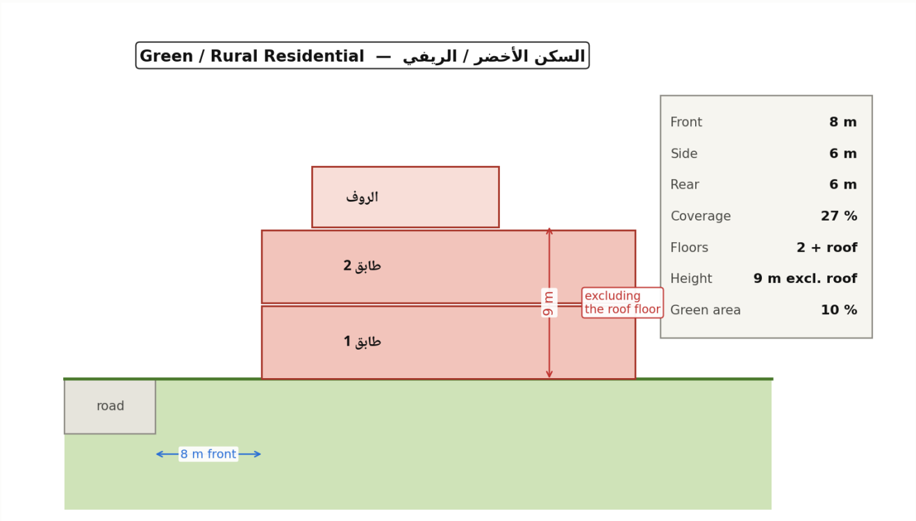
JO-Fig-15 — Development control — Green / Rural Residential · Art 16(a)
