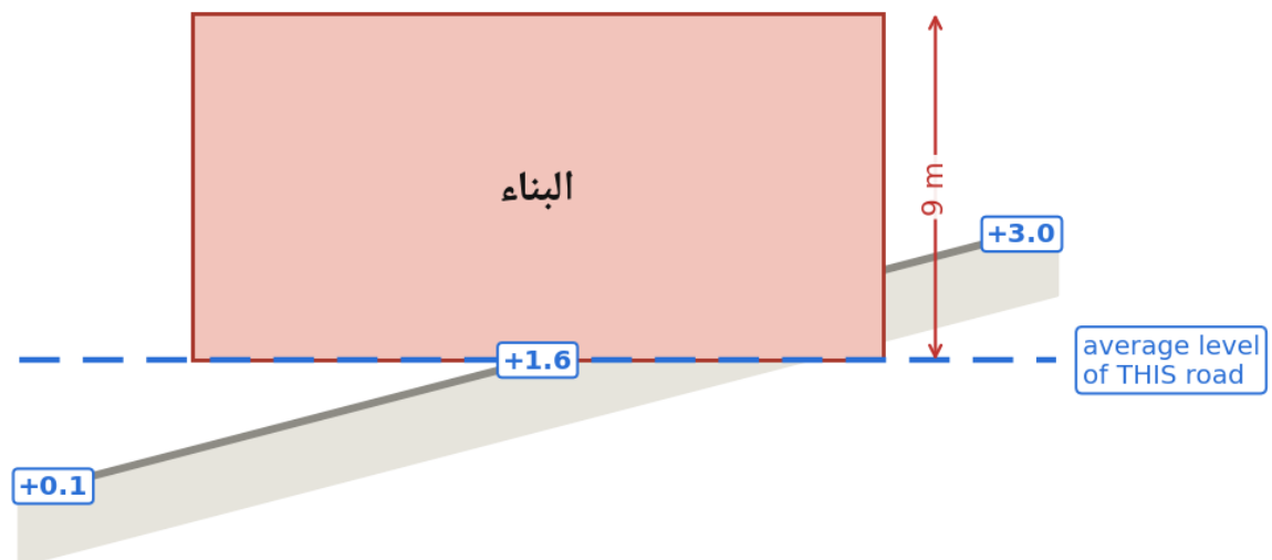
JO-Fig-09 — One road with several levels — use its average · Art 15(f)
