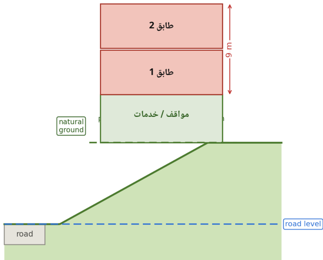
JO-Fig-07 — Natural ground above road level — the Article 15(c) relief · Art 15(c)
