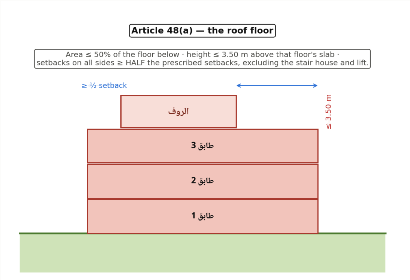
JO-Fig-29 — The roof floor — 50%, 3.50 m, half setbacks · Art 48(a)
