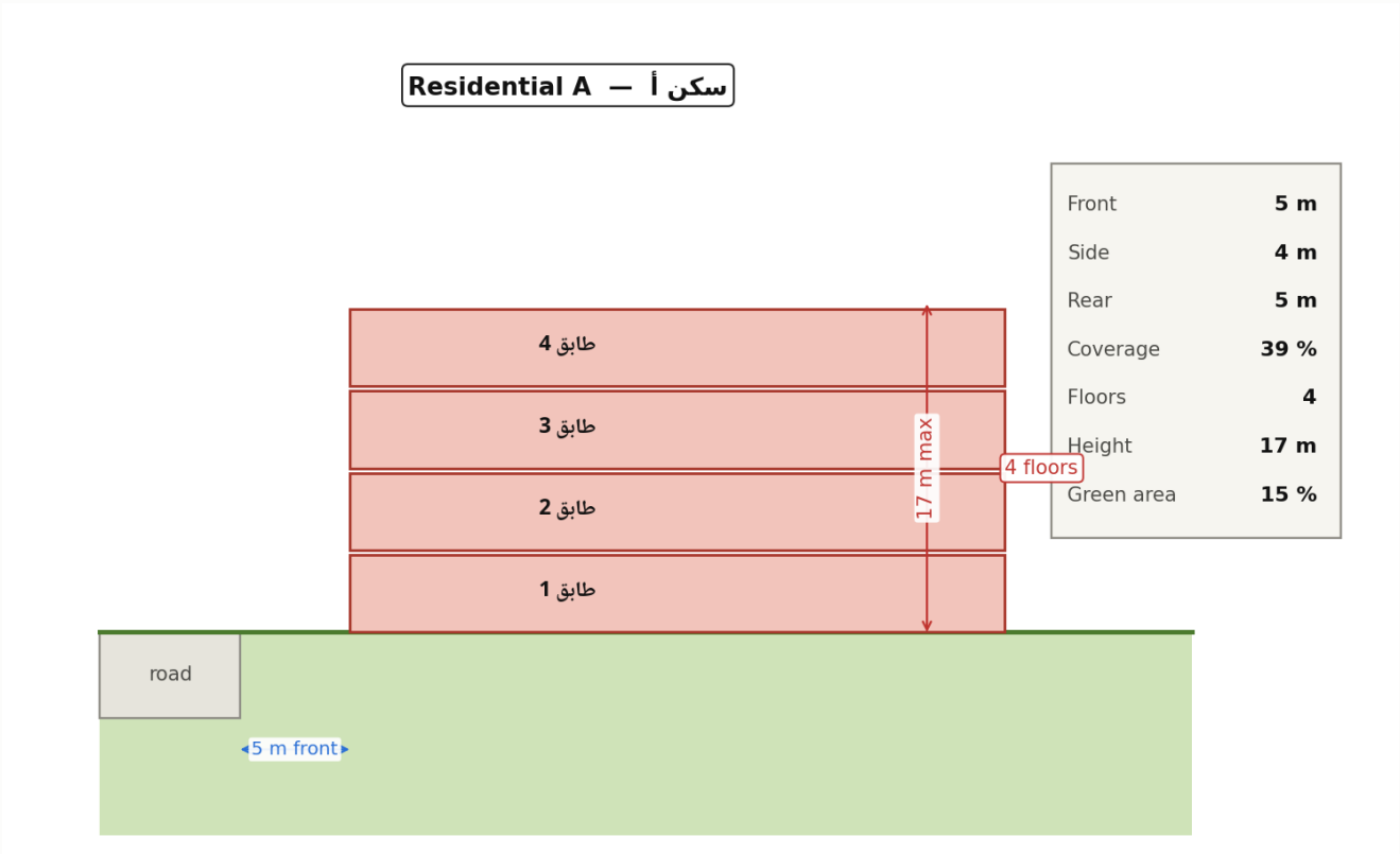
JO-Fig-14 — Development control — Residential A (سكن أ) · Art 16(a)
