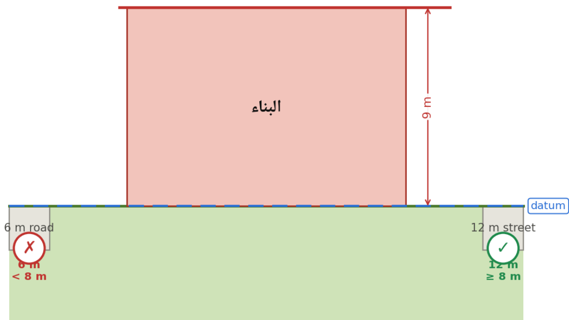
JO-Fig-04 — Height datum — roads narrower than 8 m are disregarded · Art 15(a)(1)
