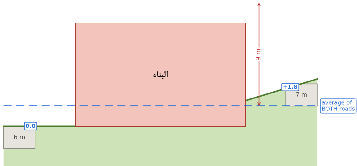
JO-Fig-05 — Where every adjoining road is under 8 m — average them · Art 15(a)(2)
