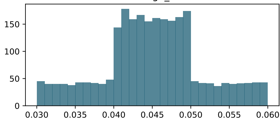
Omega_b
