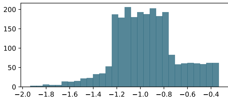
w0
