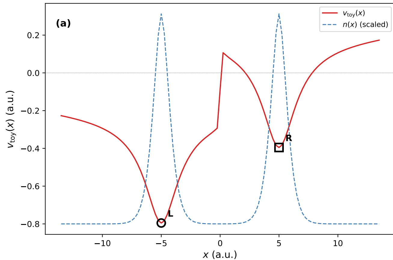
Real space ( S = 0.4 )
