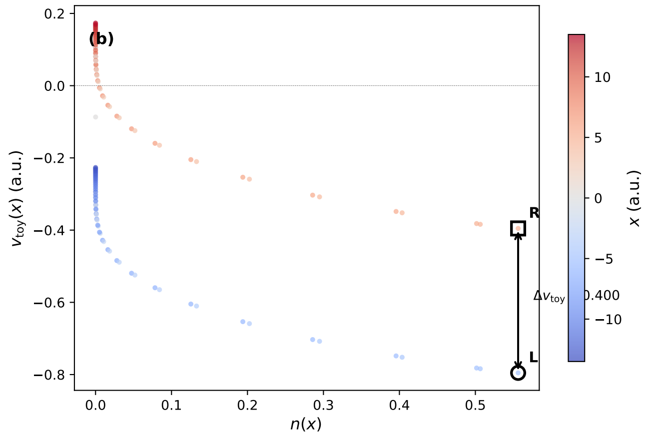
Descriptor space ( S = 0.4 )
