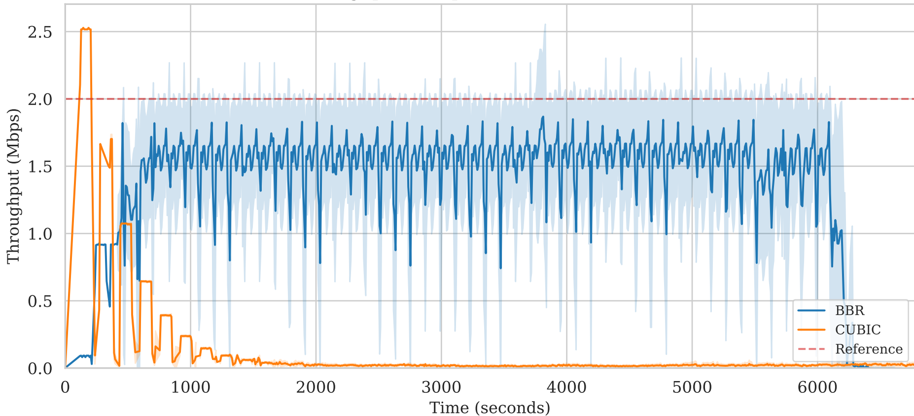
Throughput Comparison (1% Packet Loss)
