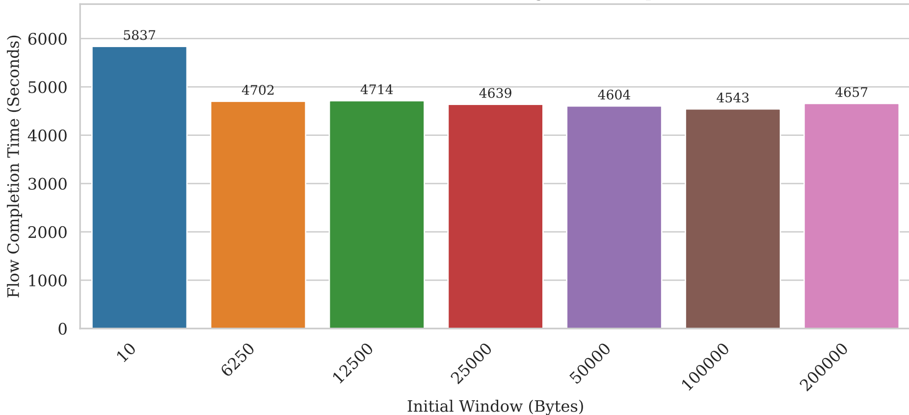
CUBIC Initial Window Tuning (FCT Comparison)
