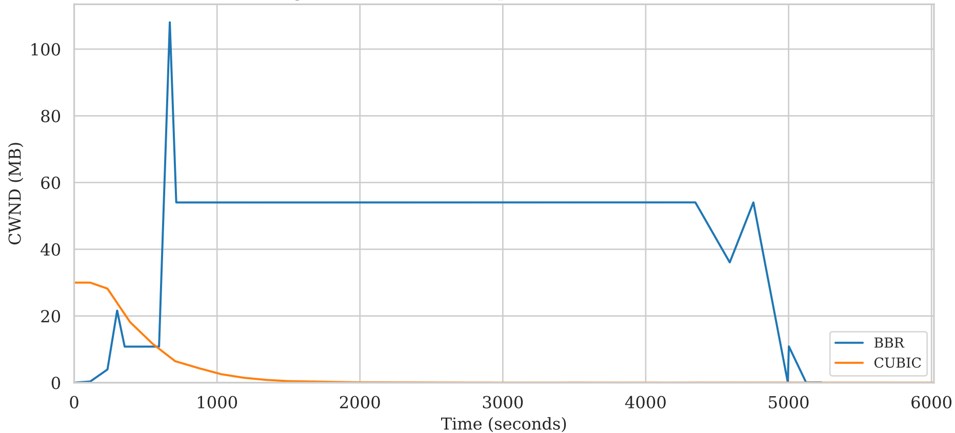
Congestion Window Comparison (10% Packet Loss)
