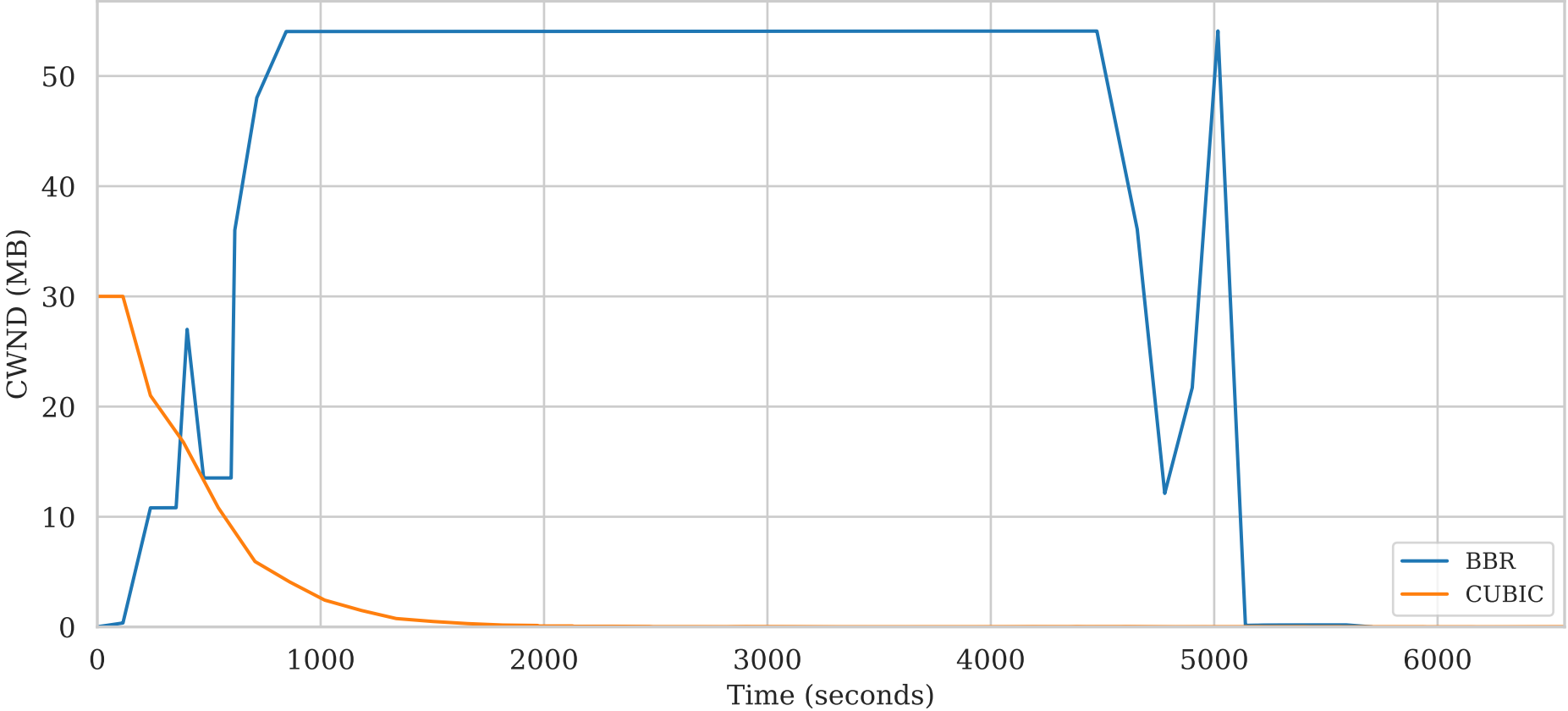
Congestion Window Comparison (20% Packet Loss)
