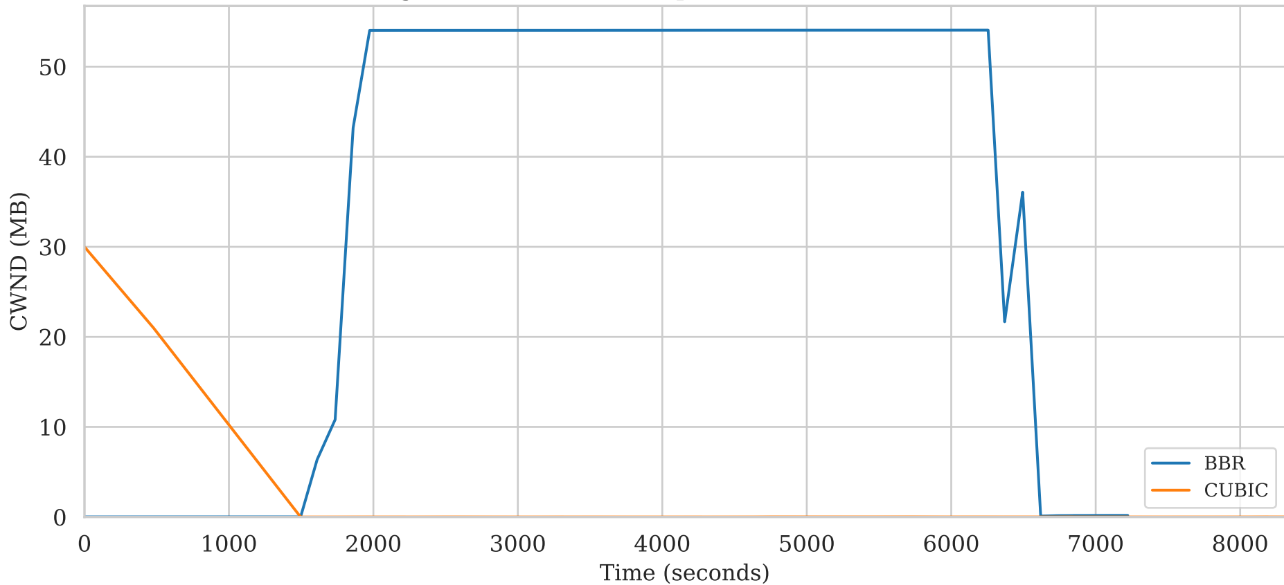
Congestion Window Comparison (30% Packet Loss)
