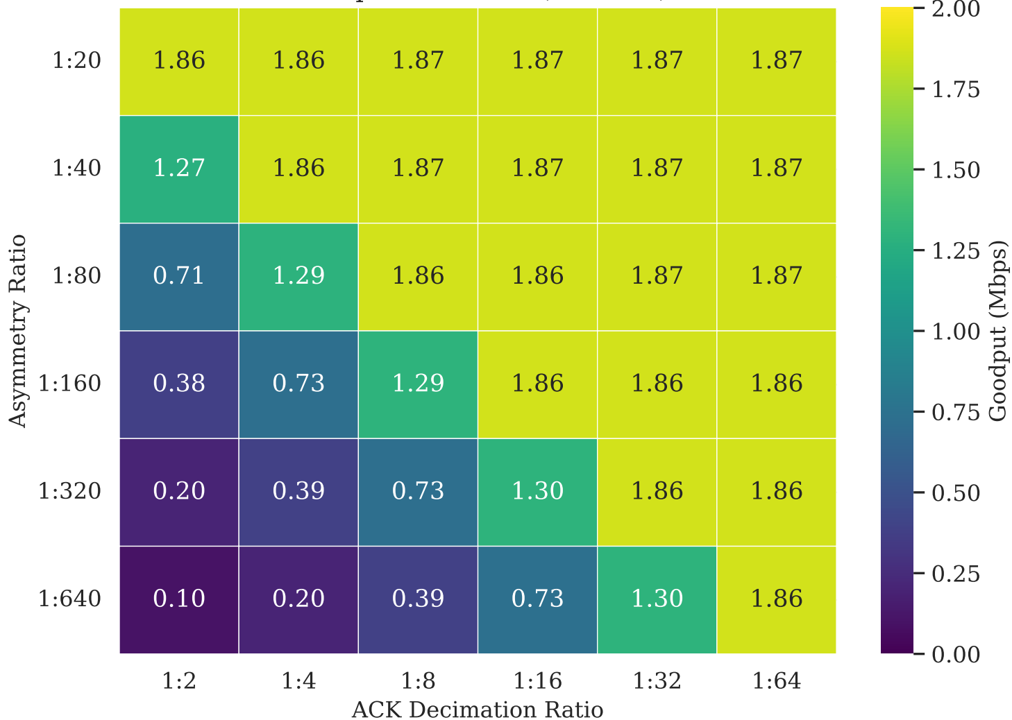
Goodput Overview (Loss 0%)
