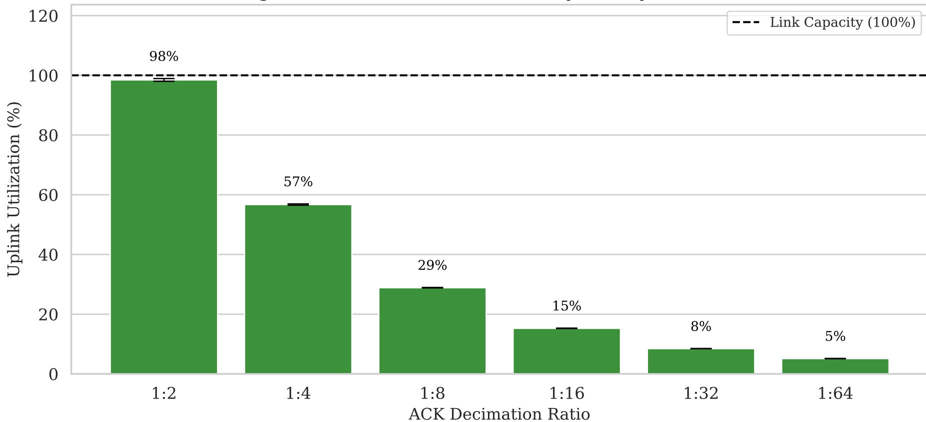
Averaged Reverse Path Saturation (Asymmetry 1:20, Loss 1%)
