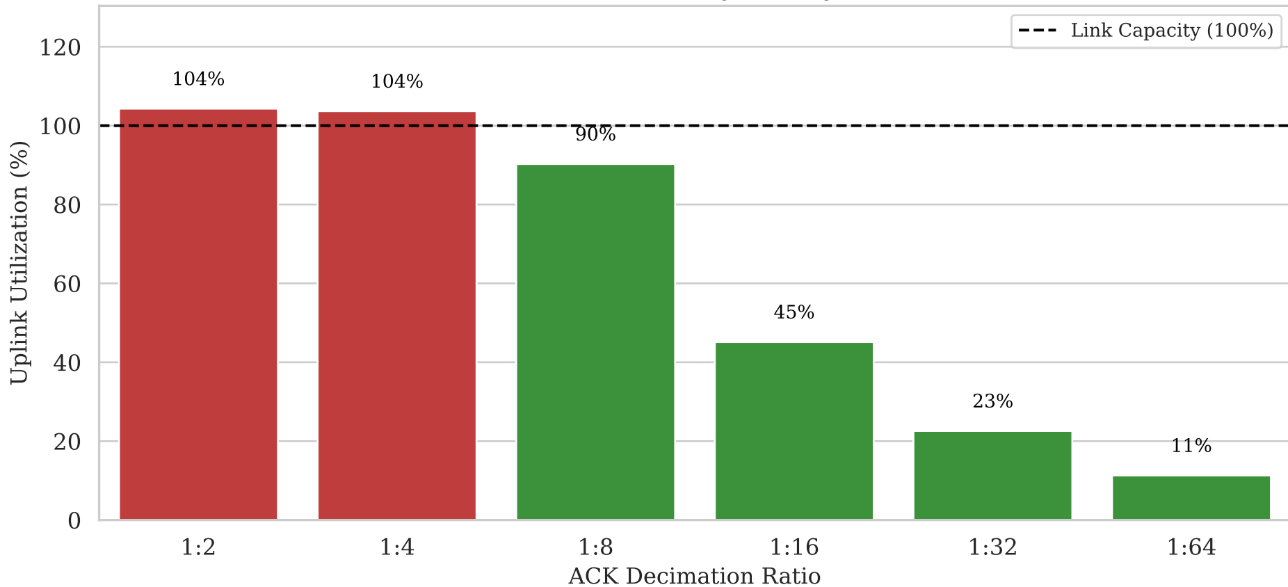
Reverse Path Saturation (Asymmetry 1:80, Loss 0%)
