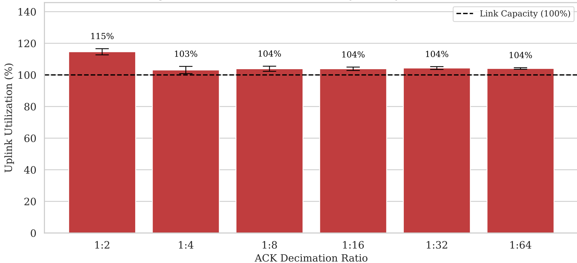
Averaged Reverse Path Saturation (Asymmetry 1:640, Loss 1%)
