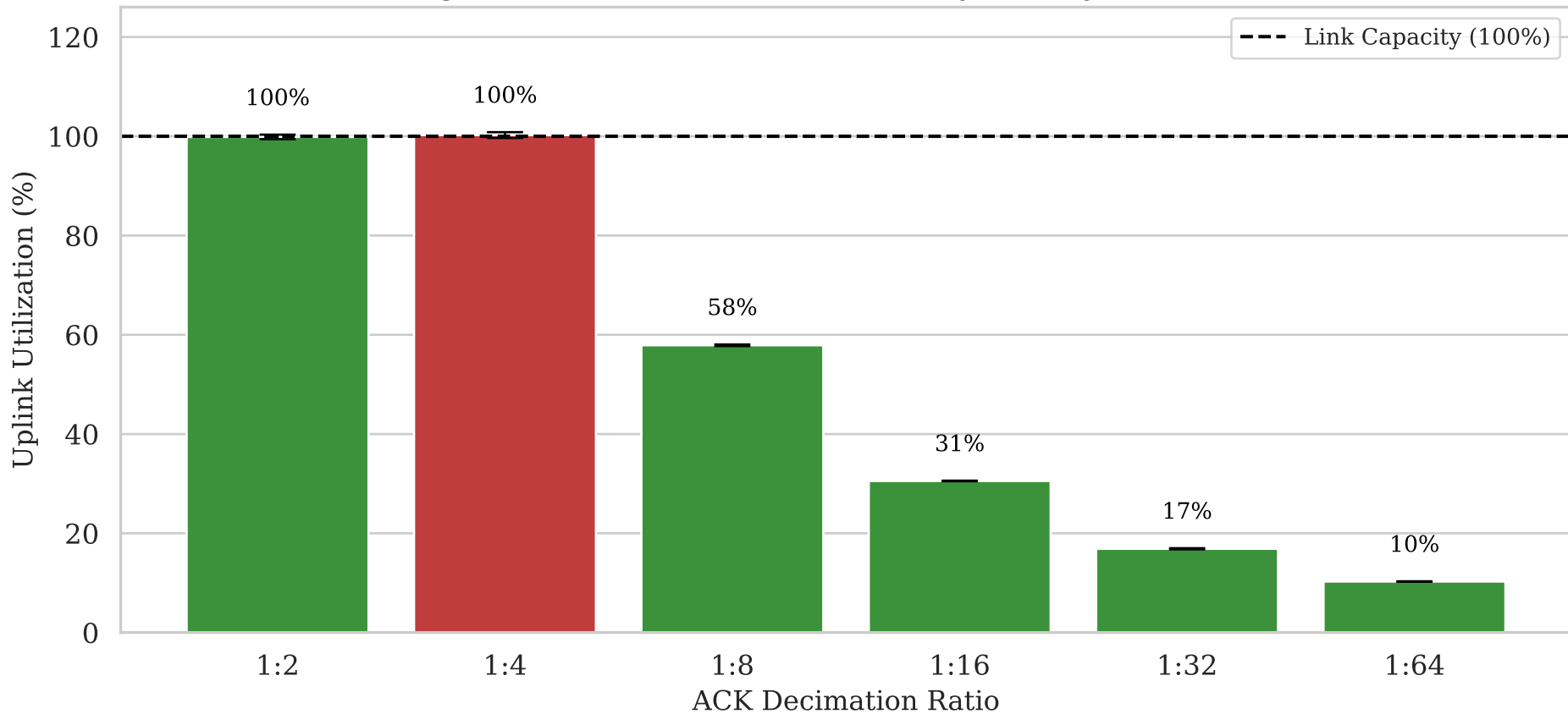
Averaged Reverse Path Saturation (Asymmetry 1:40, Loss 1%)
