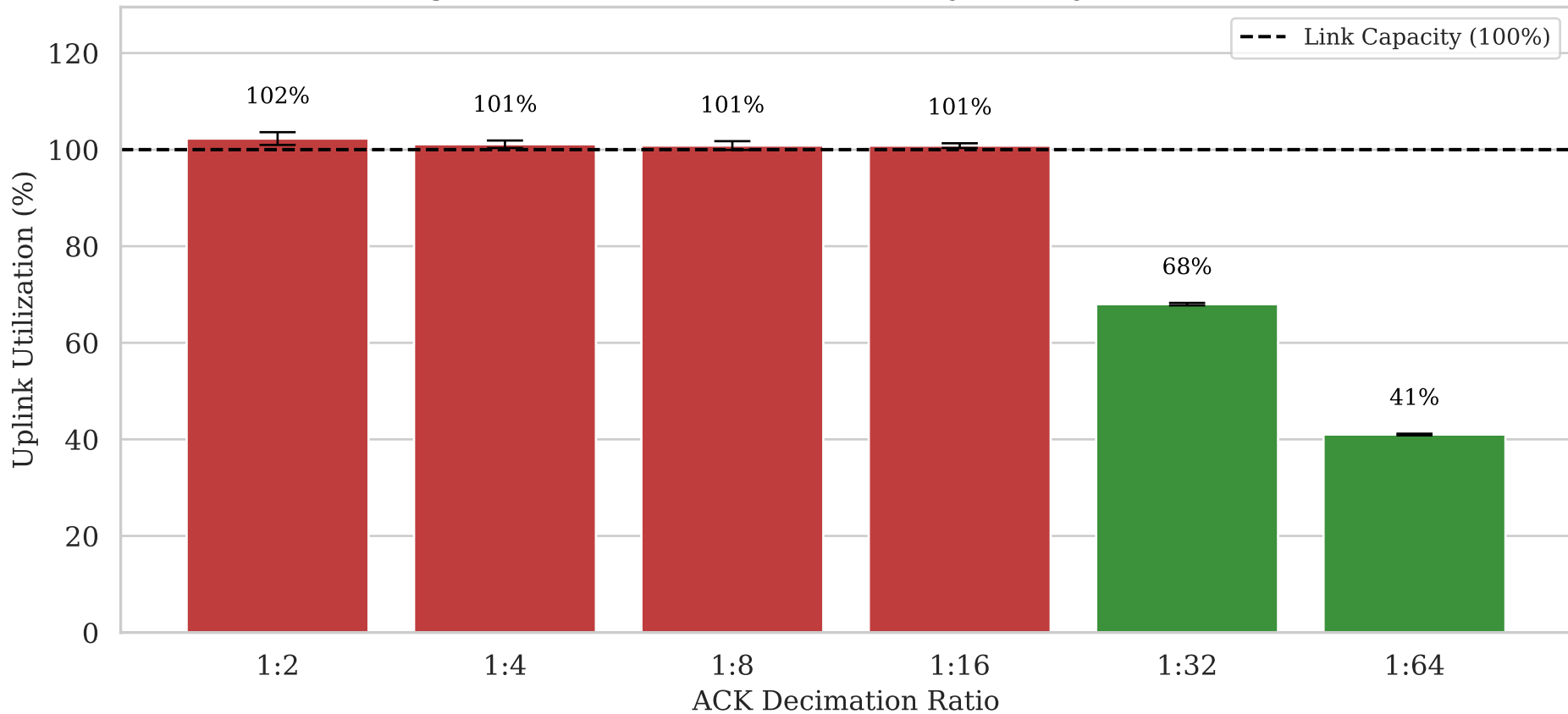
Averaged Reverse Path Saturation (Asymmetry 1:160, Loss 1%)
