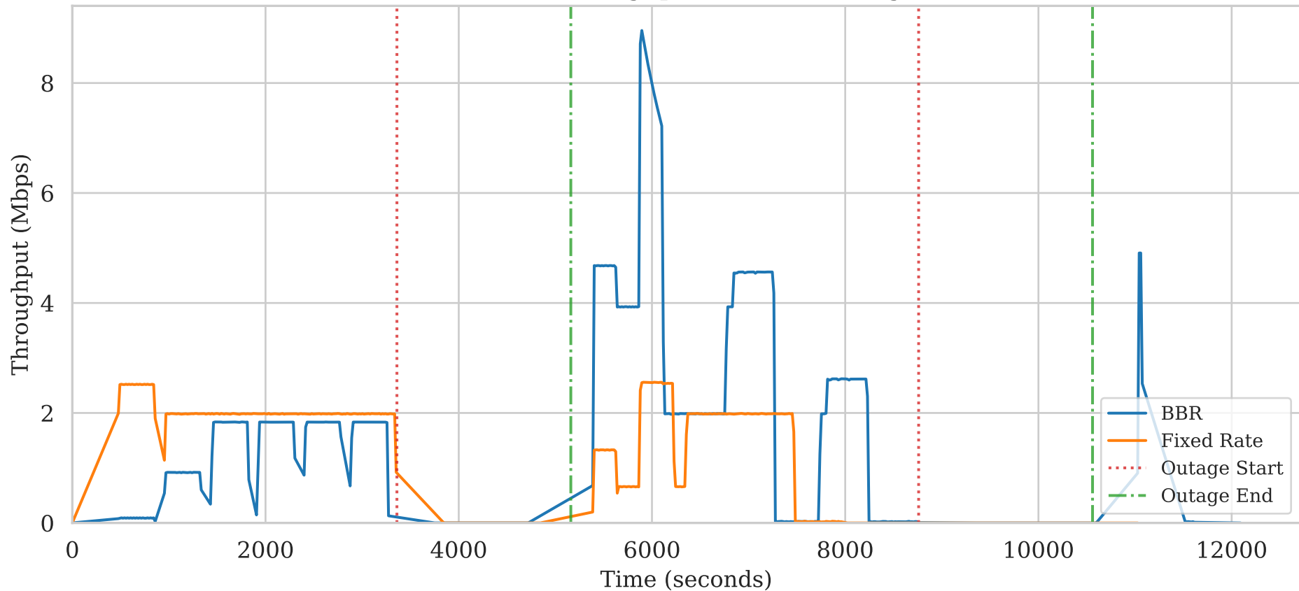
Sender Throughput (30 min Outage)
