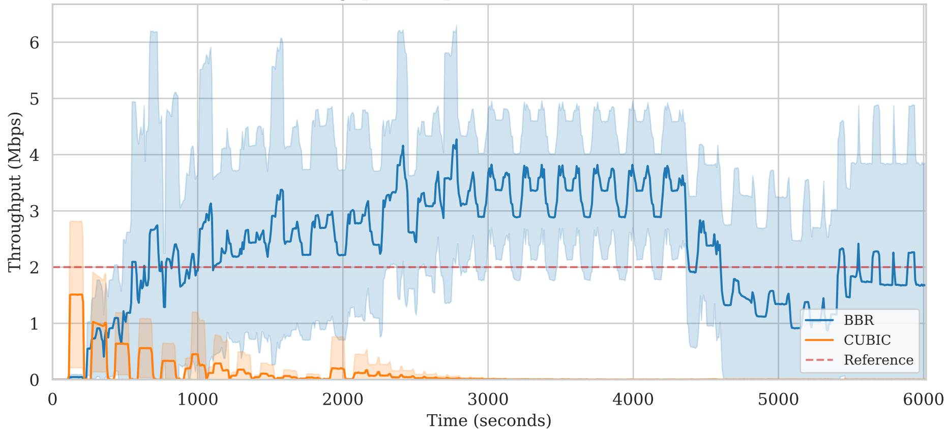
Throughput Comparison (10% Packet Loss)
