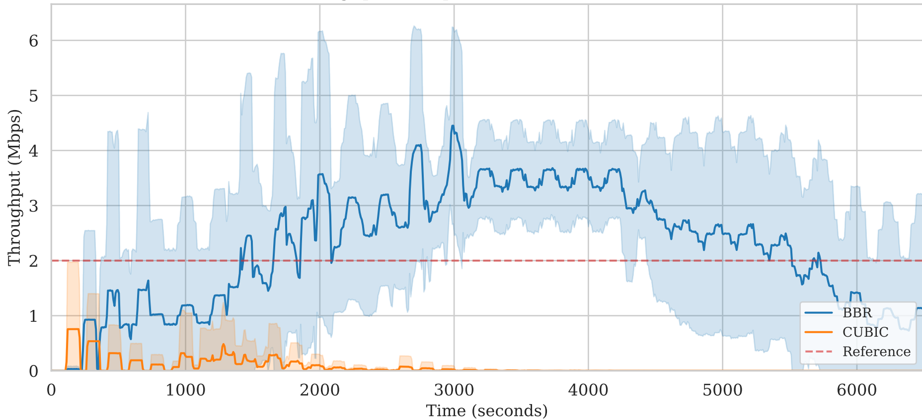
Throughput Comparison (30% Packet Loss)
