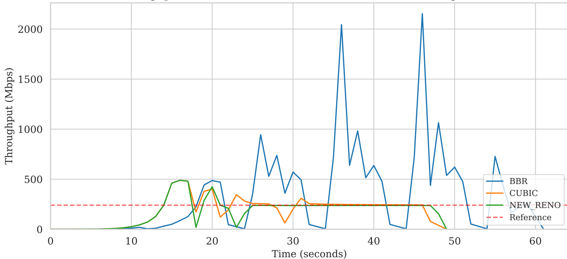
Throughput in Terrestrial Control Scenario (Default Configuration)
