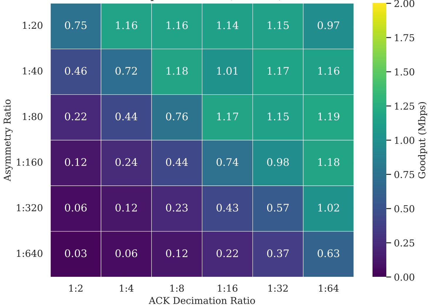
Goodput Overview (Loss 1%)
