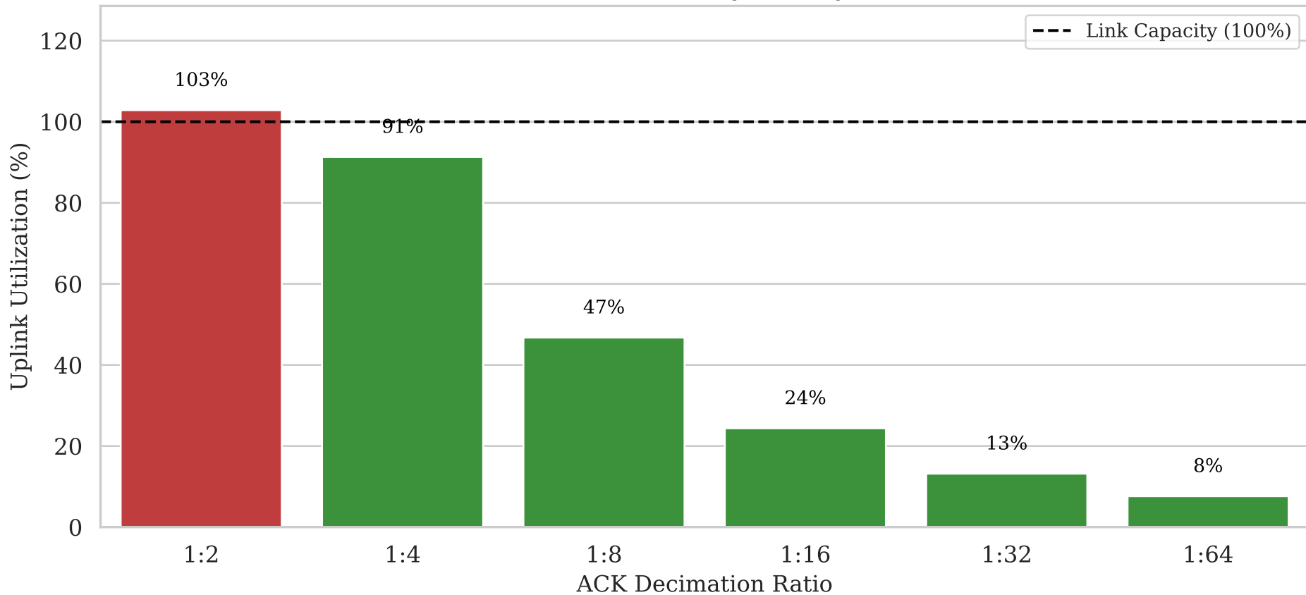
Reverse Path Saturation (Asymmetry 1:20, Loss 1%)
