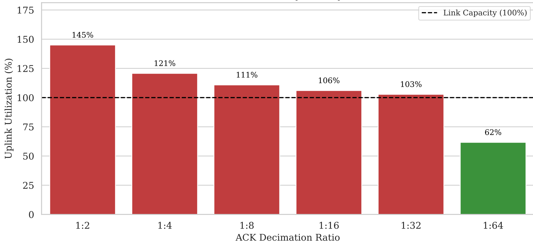
Reverse Path Saturation (Asymmetry 1:160, Loss 1%)
