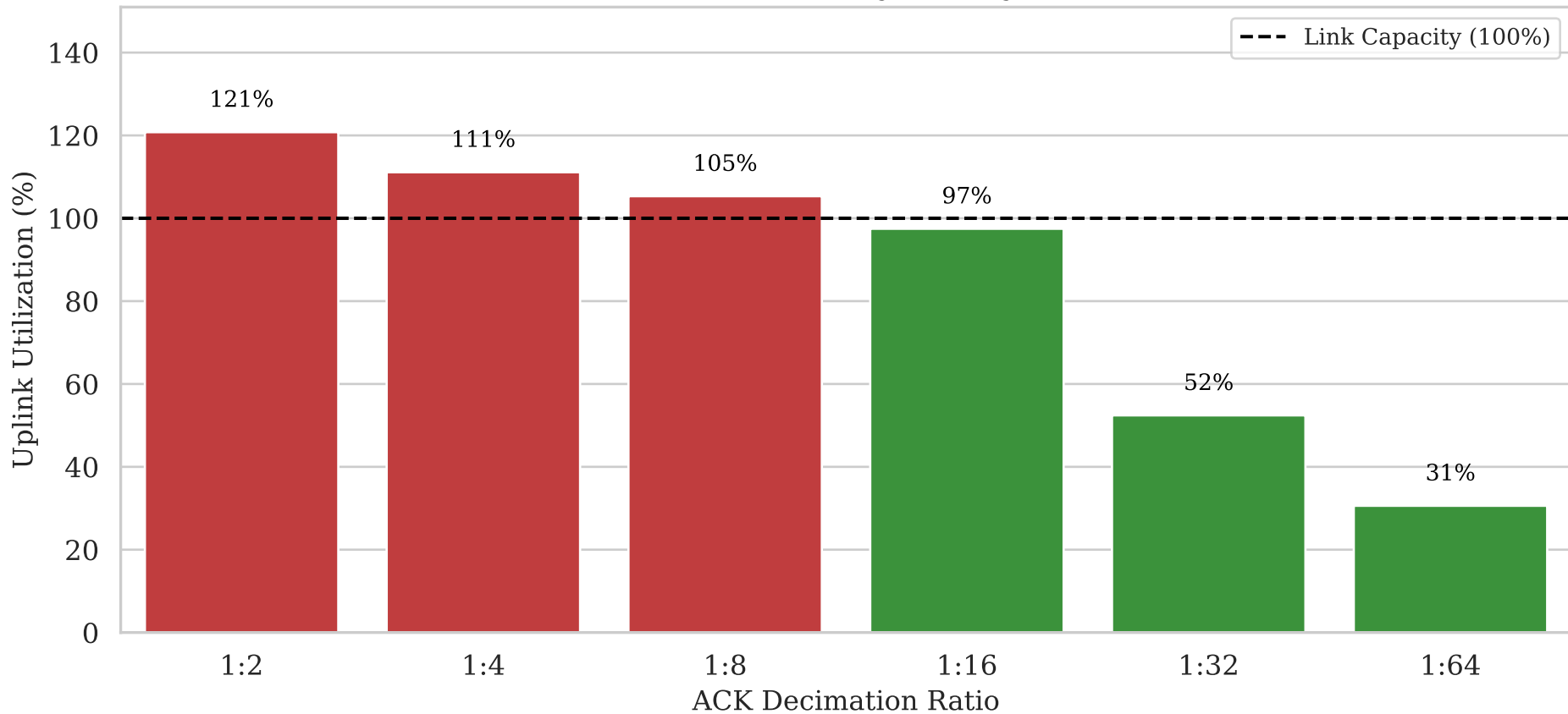
Reverse Path Saturation (Asymmetry 1:80, Loss 1%)
