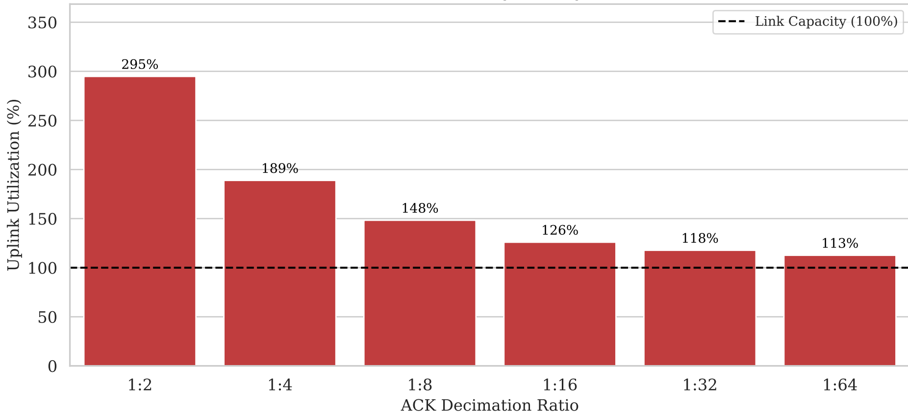
Reverse Path Saturation (Asymmetry 1:640, Loss 1%)
