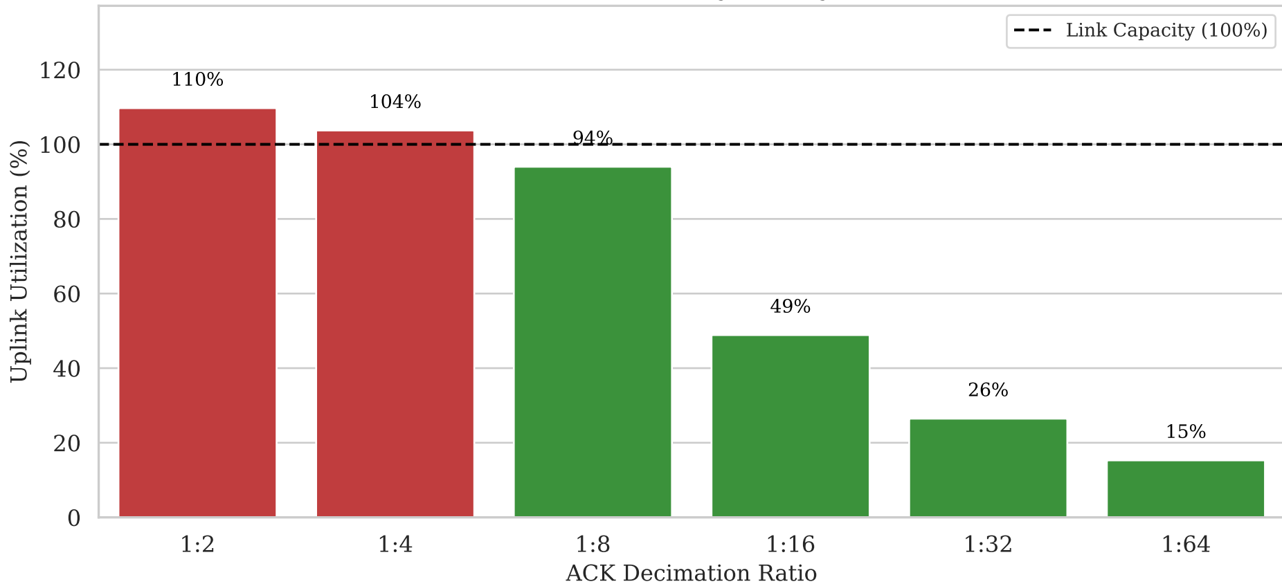
Reverse Path Saturation (Asymmetry 1:40, Loss 1%)
