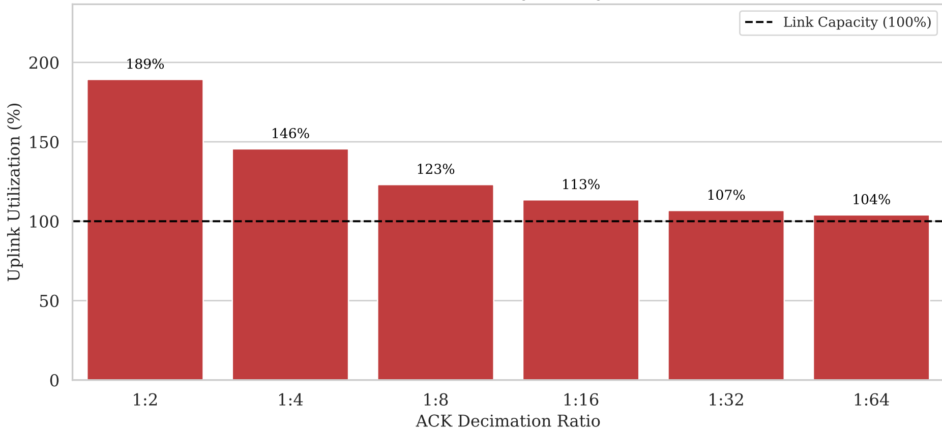
Reverse Path Saturation (Asymmetry 1:320, Loss 1%)
