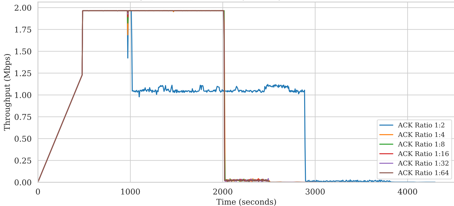
Throughput Comparison (Asymmetry Ratio 1:20, Loss 1%)
