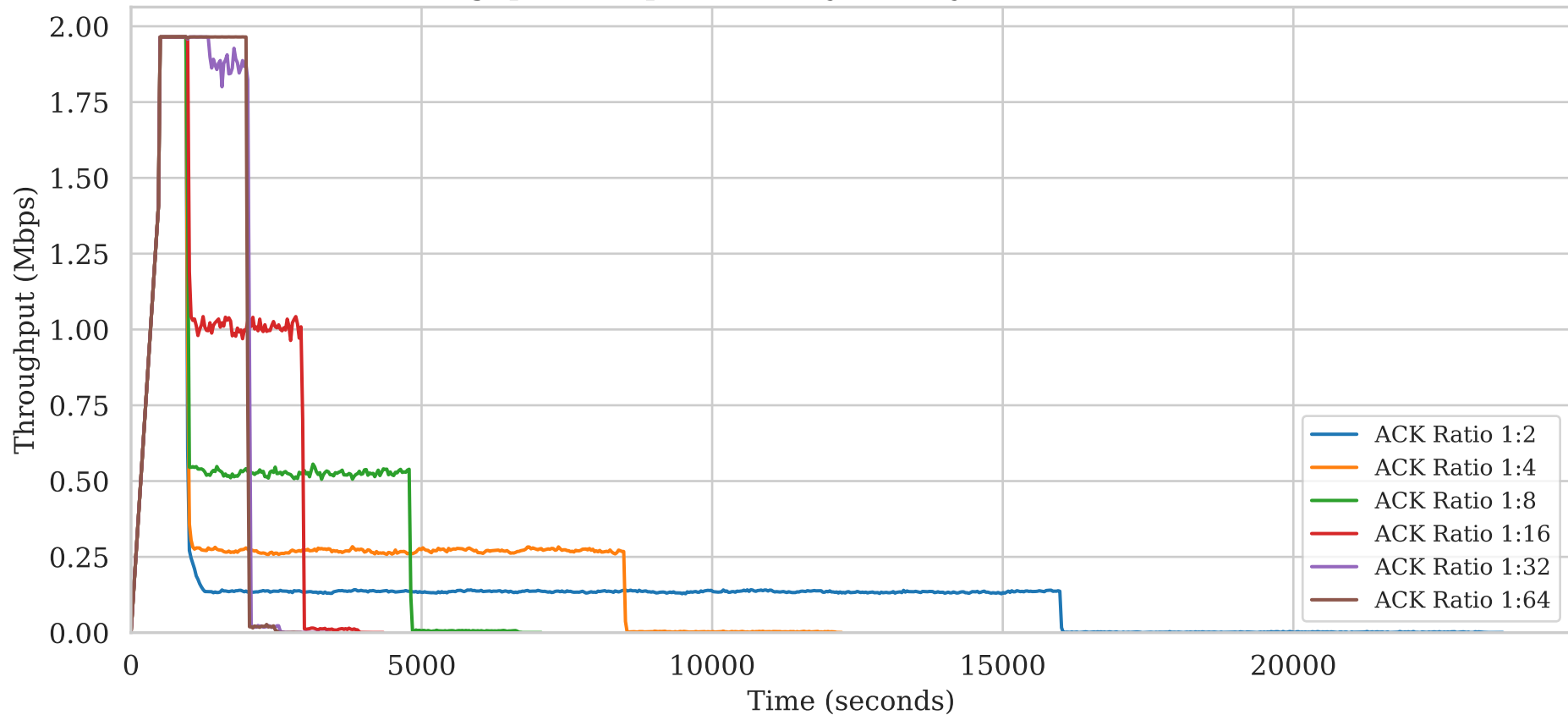
Throughput Comparison (Asymmetry Ratio 1:160, Loss 1%)
