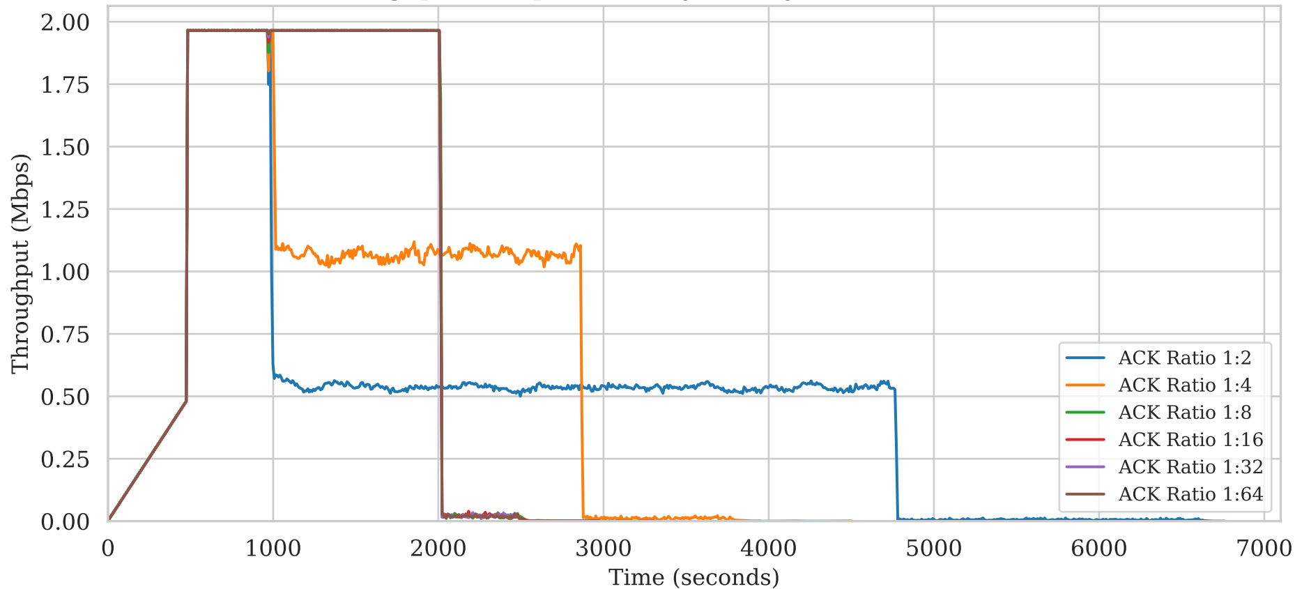
Throughput Comparison (Asymmetry Ratio 1:40, Loss 1%)
