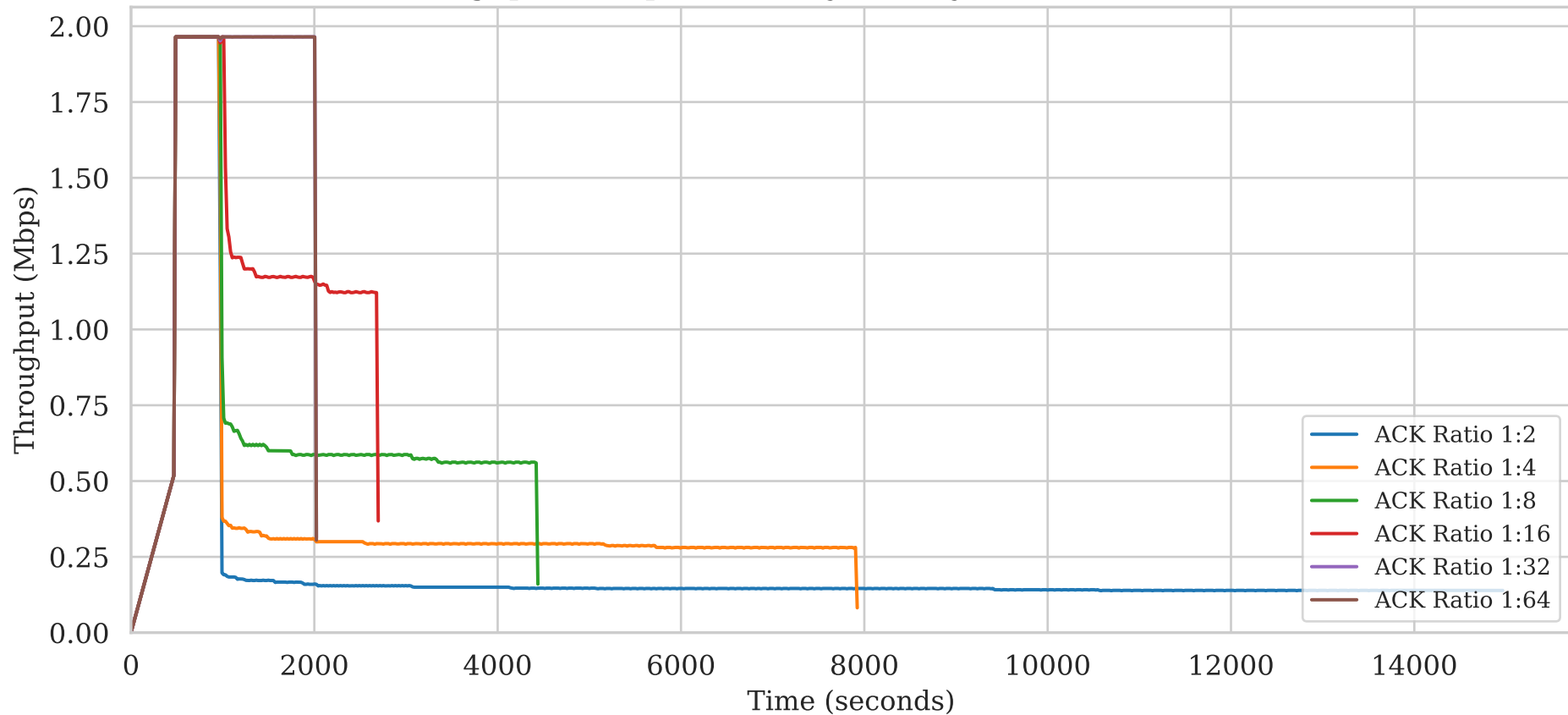
Throughput Comparison (Asymmetry Ratio 1:320, Loss 0%)
