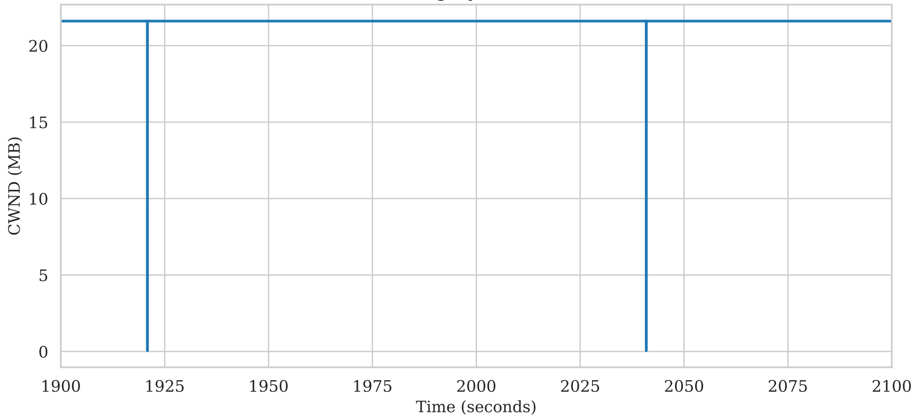
BBR CWND Probing Dynamics (1900s - 2100s)
