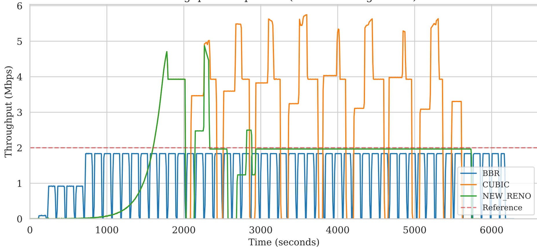
Throughput Comparison (Default Configuration)
