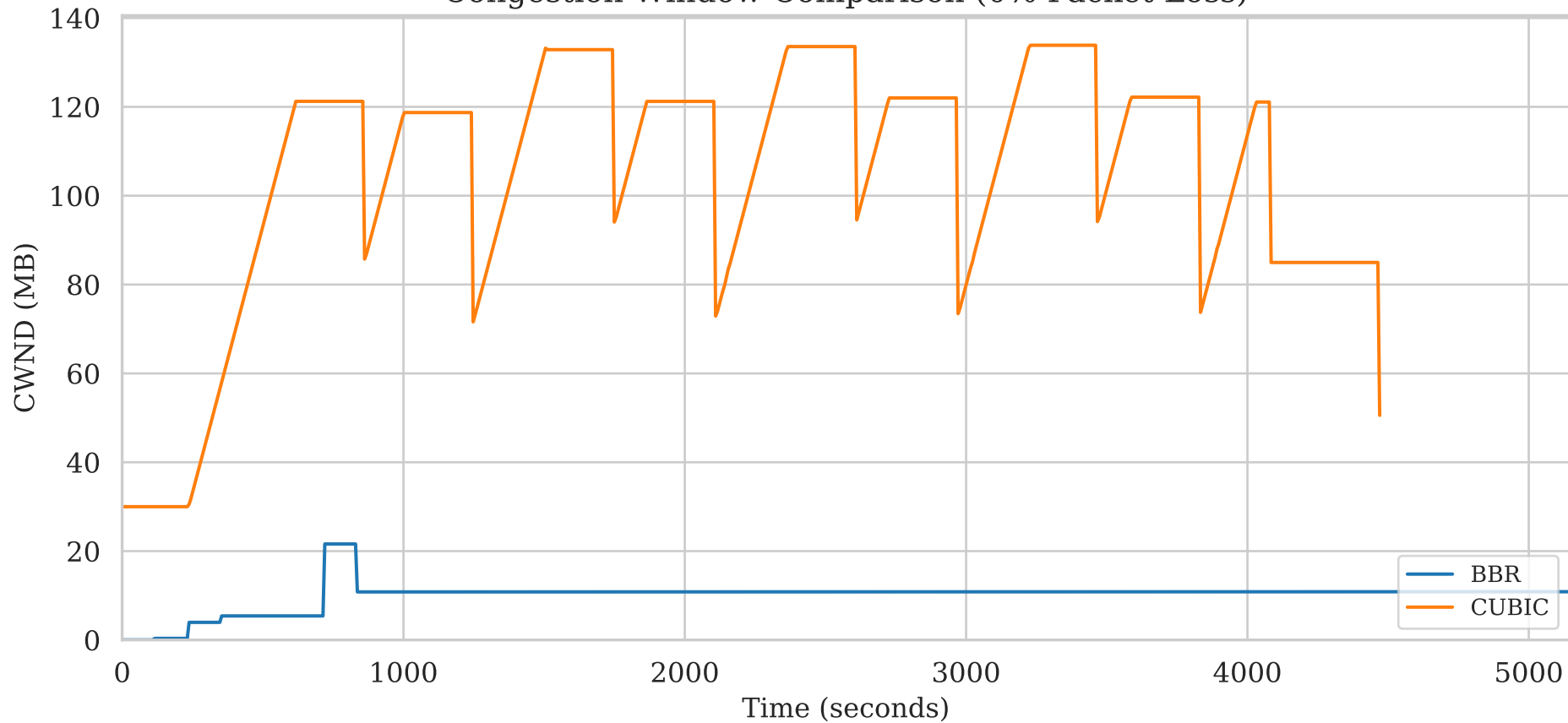
Congestion Window Comparison (0% Packet Loss)
