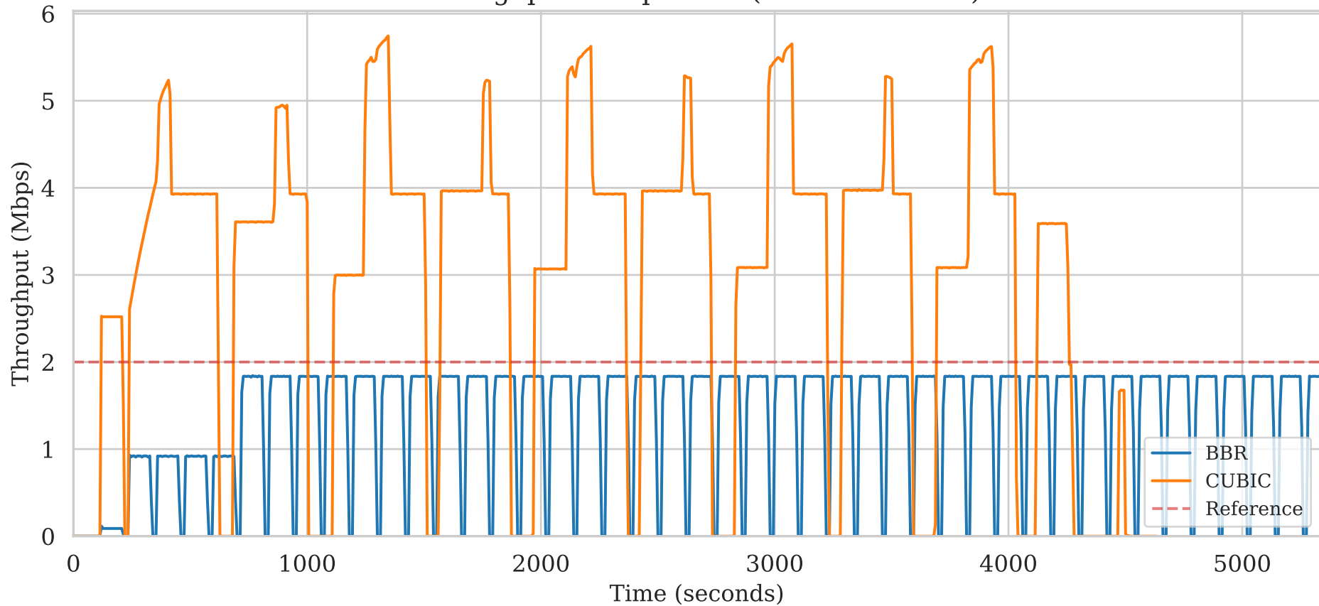
Throughput Comparison (0% Packet Loss)
