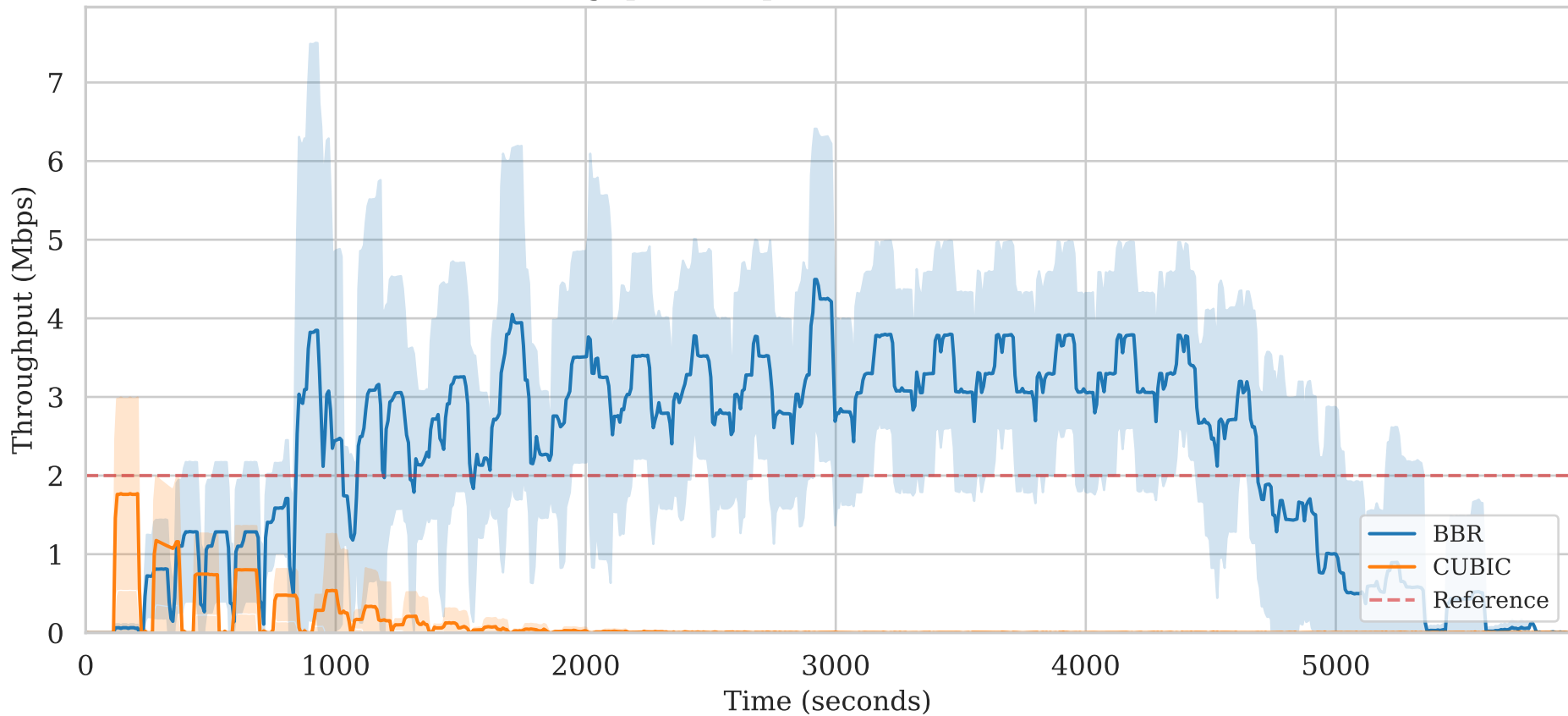
Throughput Comparison (5% Packet Loss)
