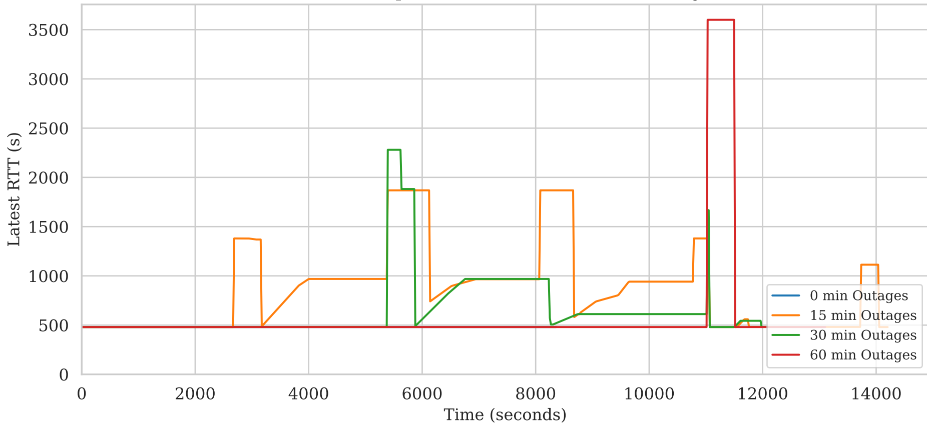
RTT Comparison: BBR with Intermittency
