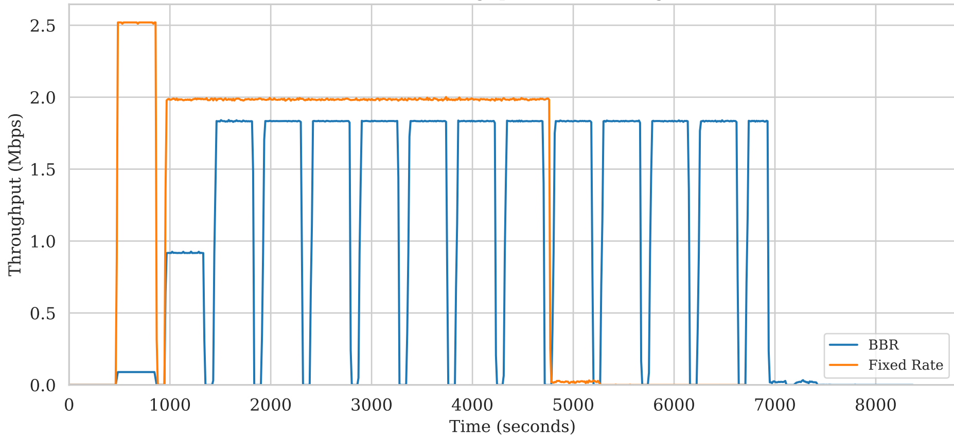
Sender Throughput (0 min Outage)
