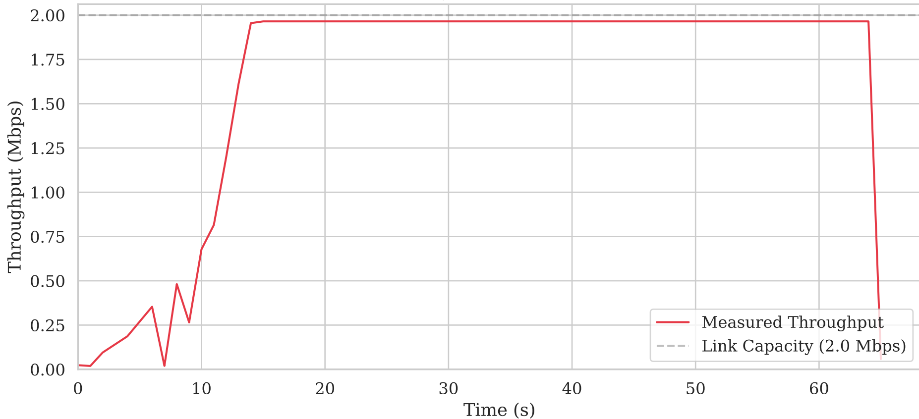
Channel Capacity Verification (2.0 Mbps Link)
