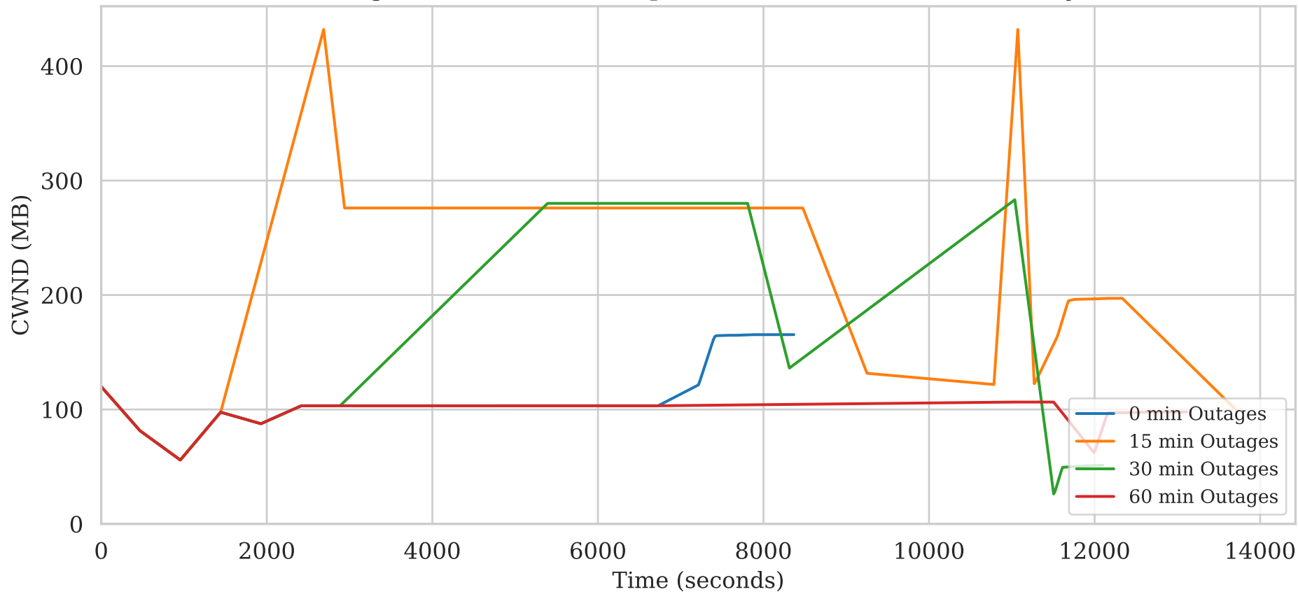
Congestion Window Comparison: BBR with Intermittency
