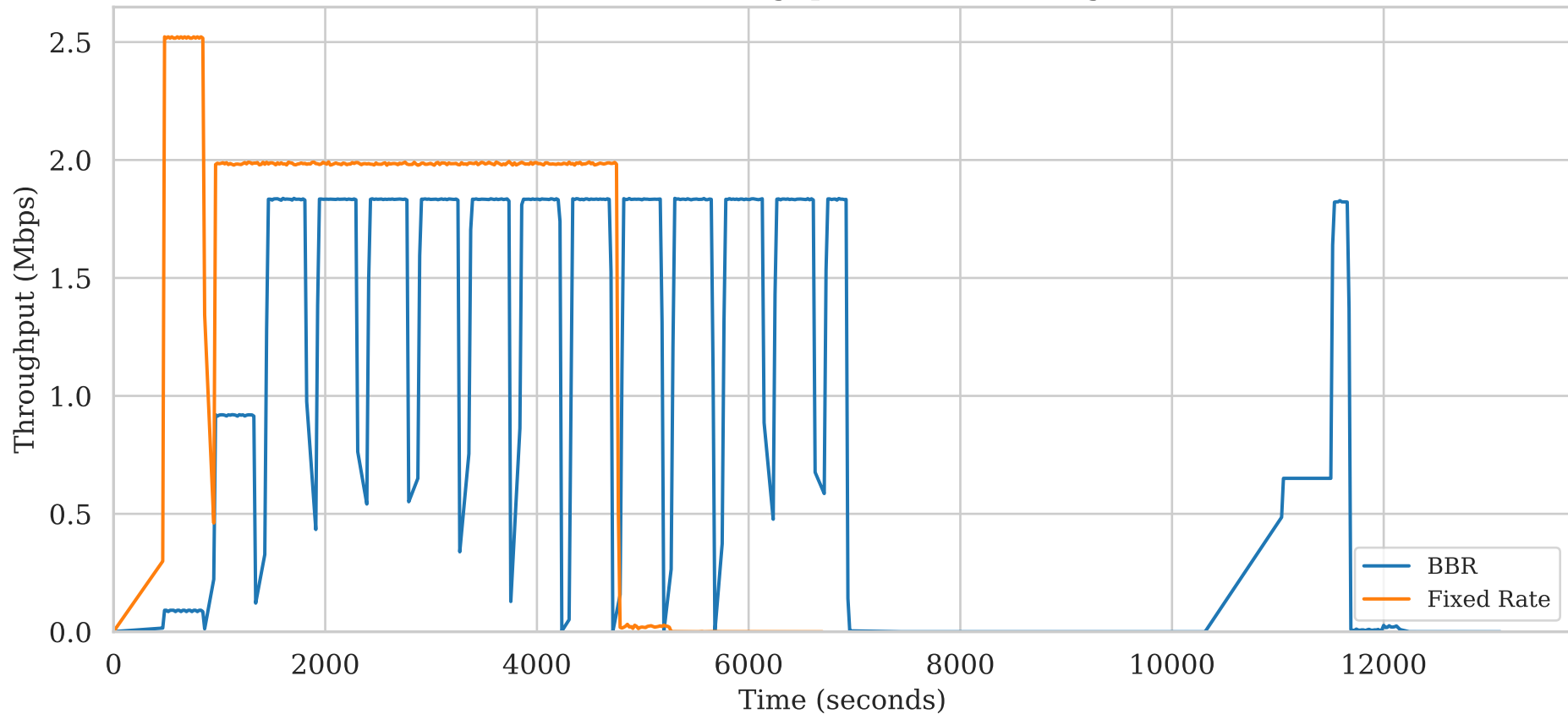
Sender Throughput (60 min Outage)
