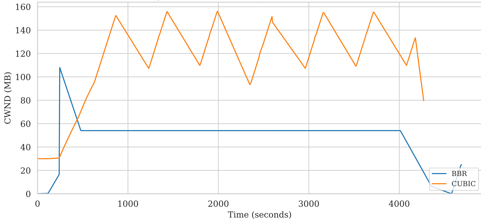
Congestion Window Comparison (0% Packet Loss)
