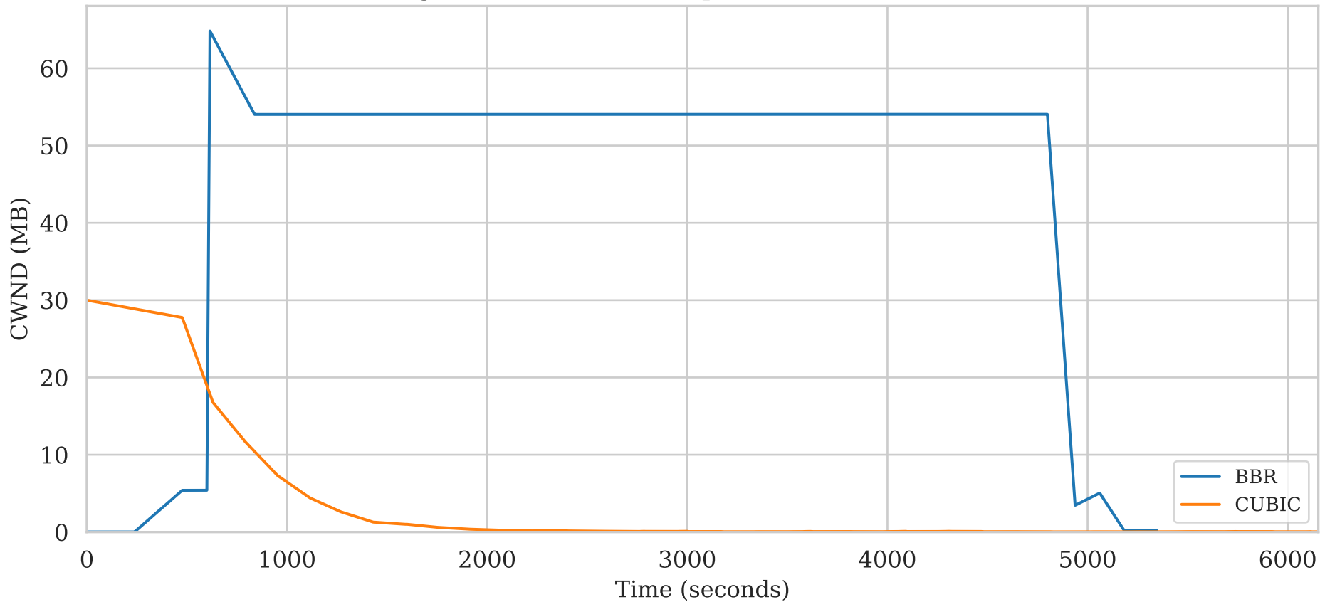
Congestion Window Comparison (5% Packet Loss)
