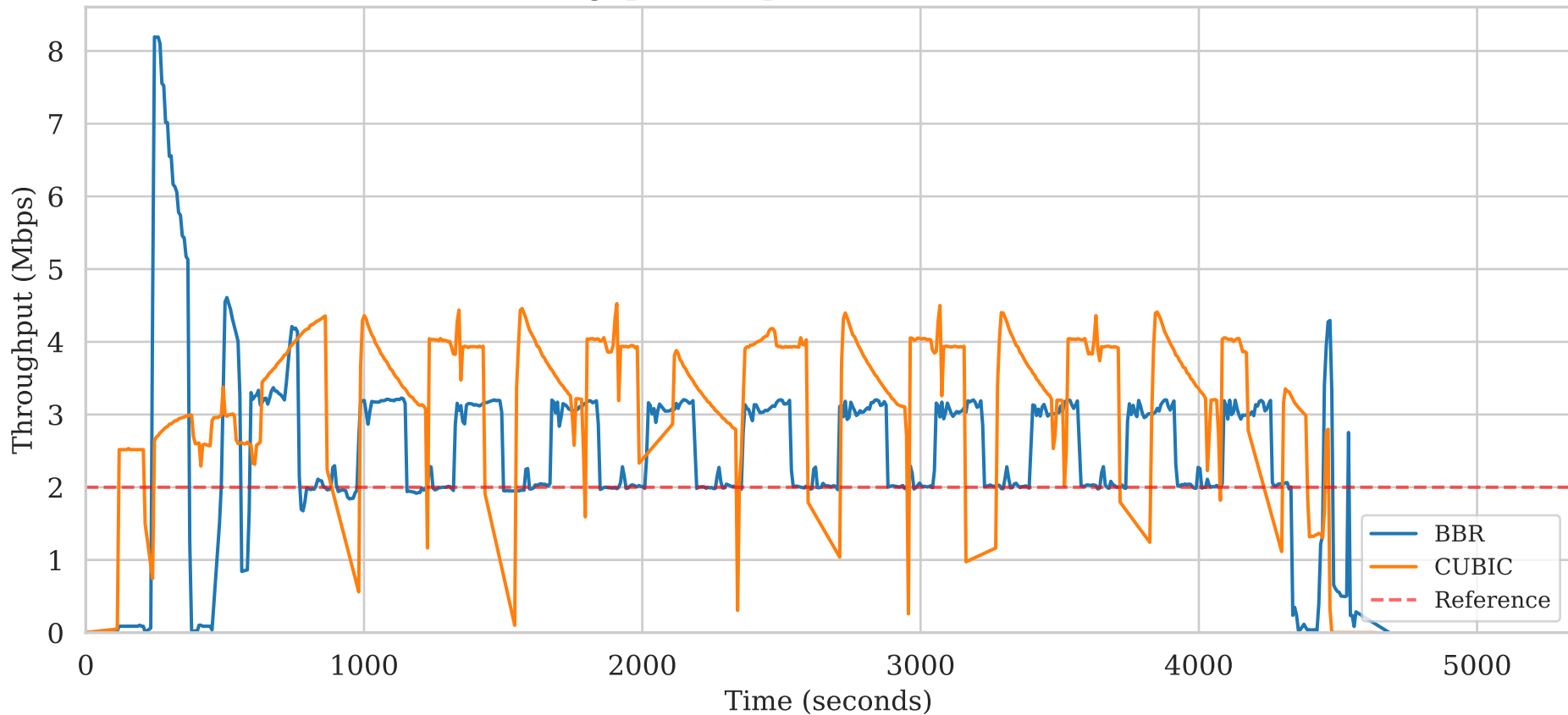
Throughput Comparison (0% Packet Loss)
